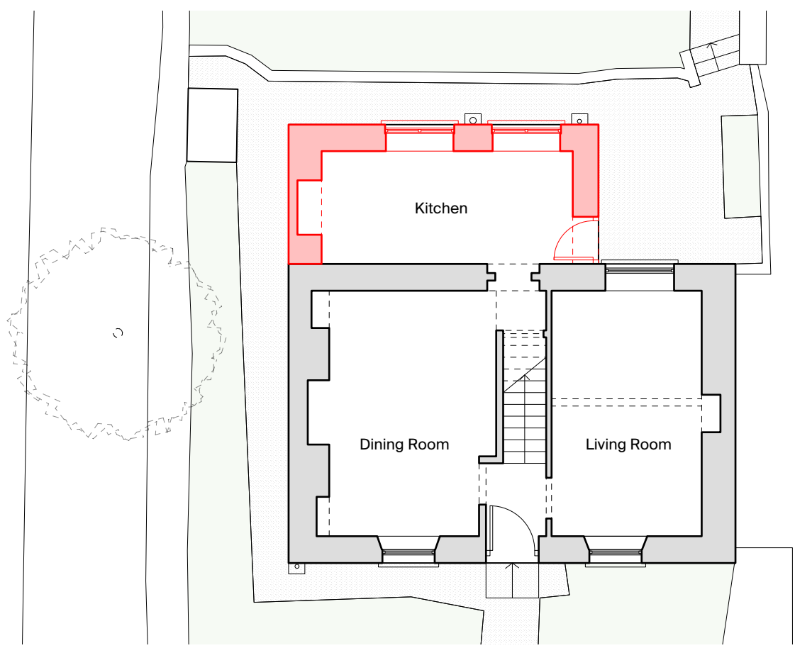
01 Existing Ground Floor Plan
