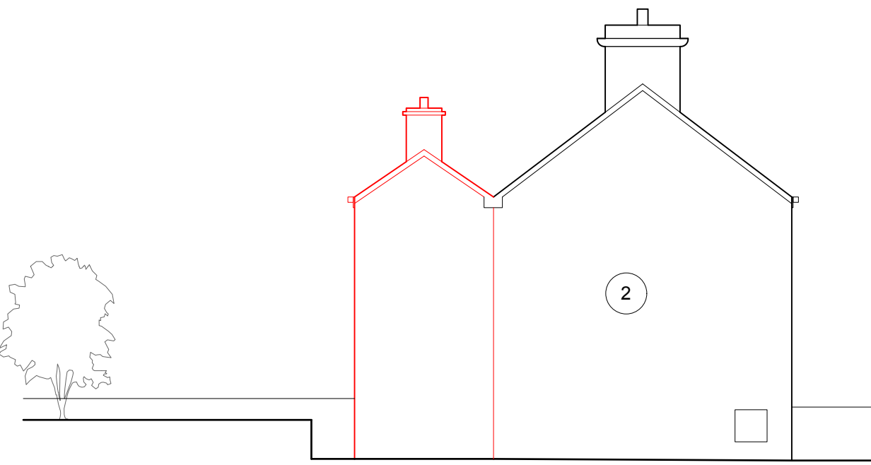
09 Existing South Elevation
