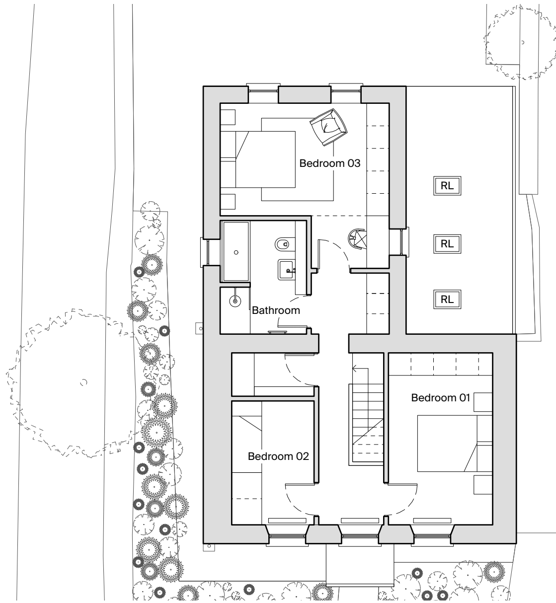
05 Proposed First Floor Plan
