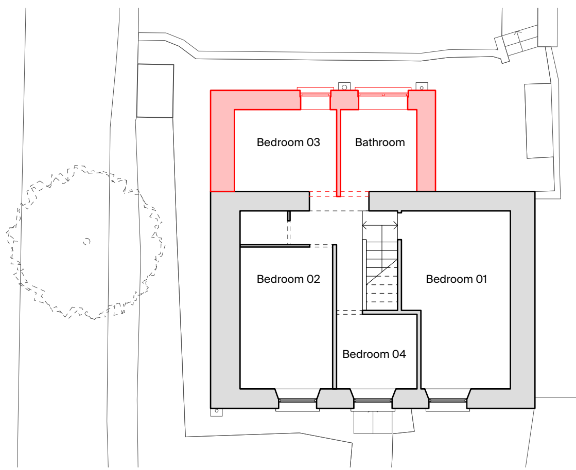
02 Existing First Floor Plan
