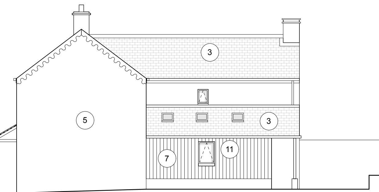
11 Proposed North Elevation
