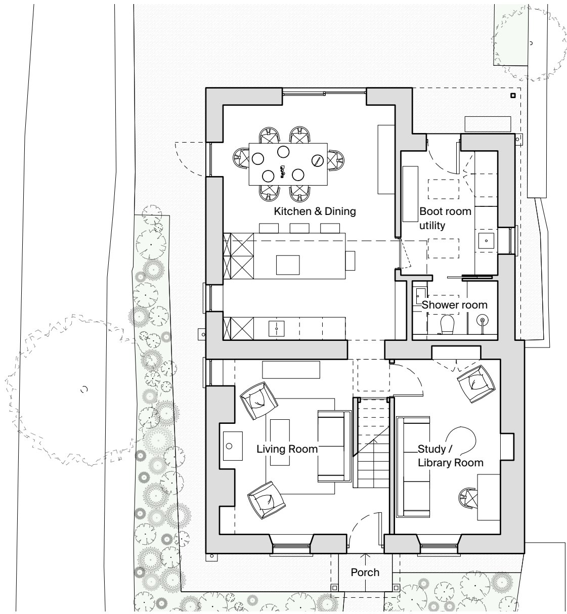
04 Proposed Ground Floor Plan
