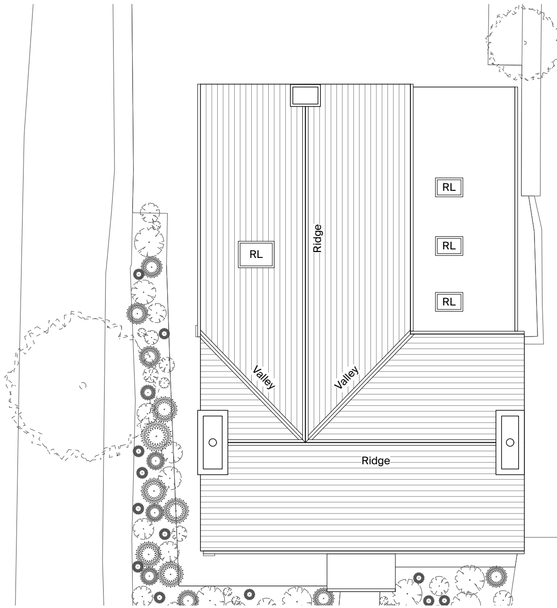
06 Proposed Roof Plan
