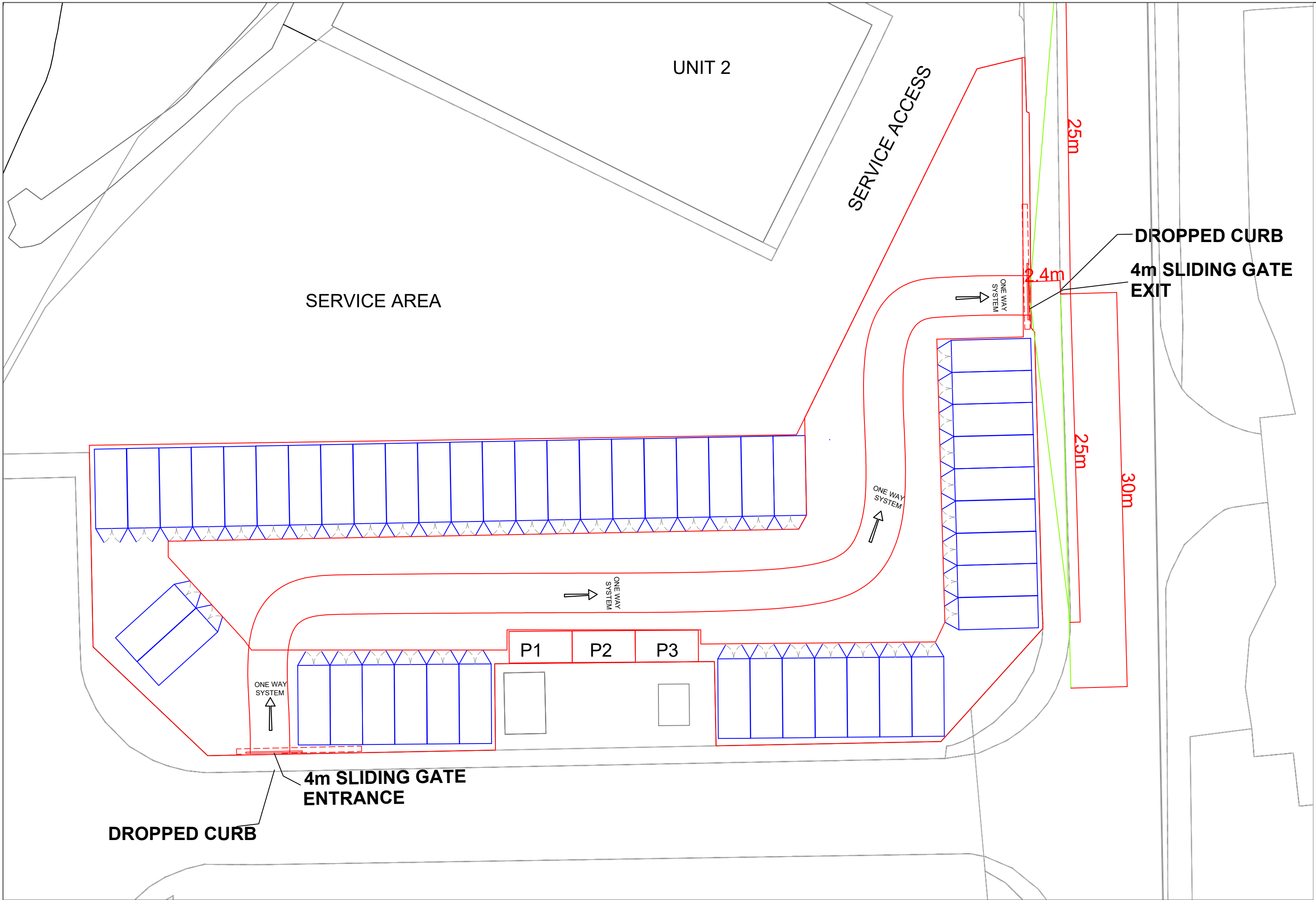
Proposed Site Layout - Scale 1/250
