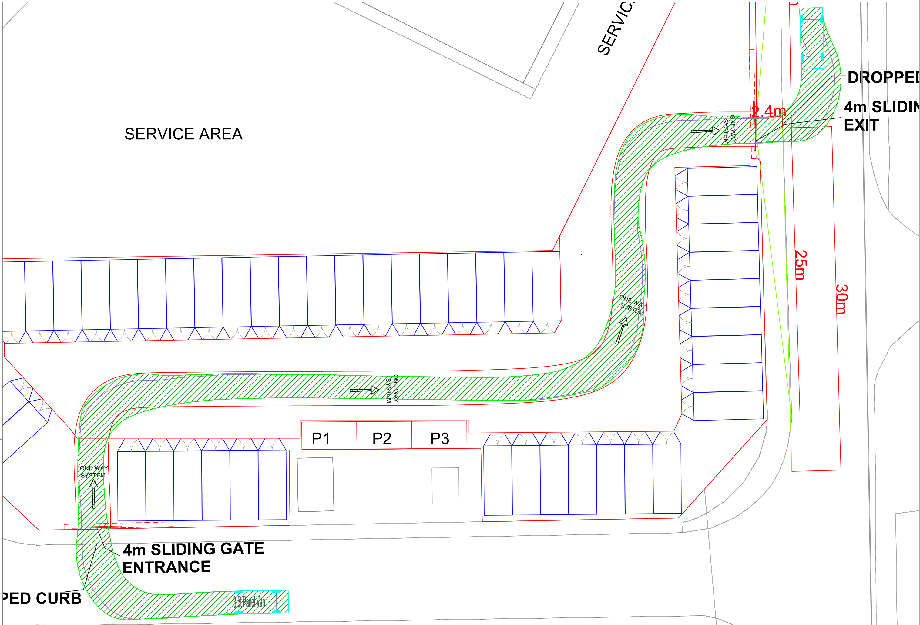
Swept Path Analysis - 3.5t Panel Van - Scale 1/200
