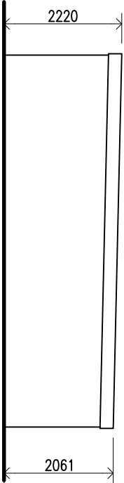
EXISTING SIDE SECTIONAL ELEVATION. (1:100)
