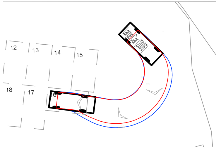
LARGE CAR ENTERING SPACE 16
