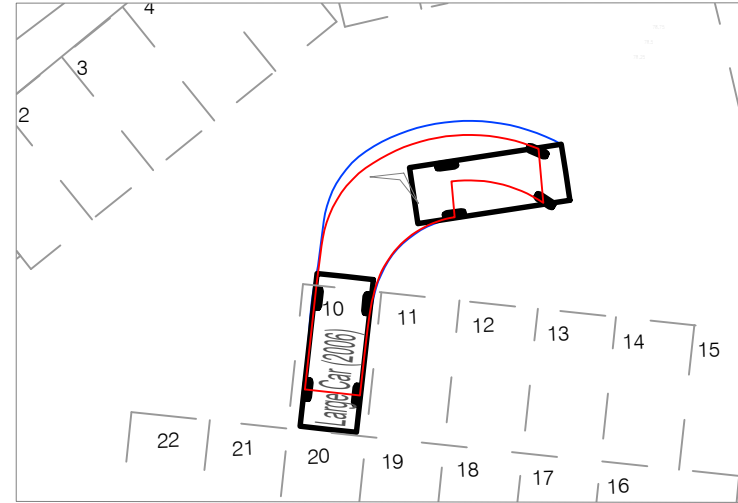
LARGE CAR EXITING SPACE 10
