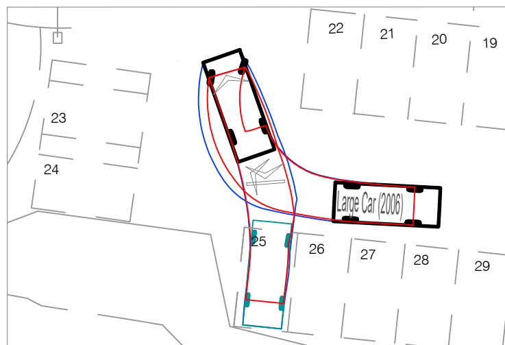
LARGE CAR ENTERING SPACE 25
