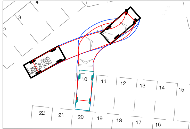
LARGE CAR ENTERING SPACE 10
