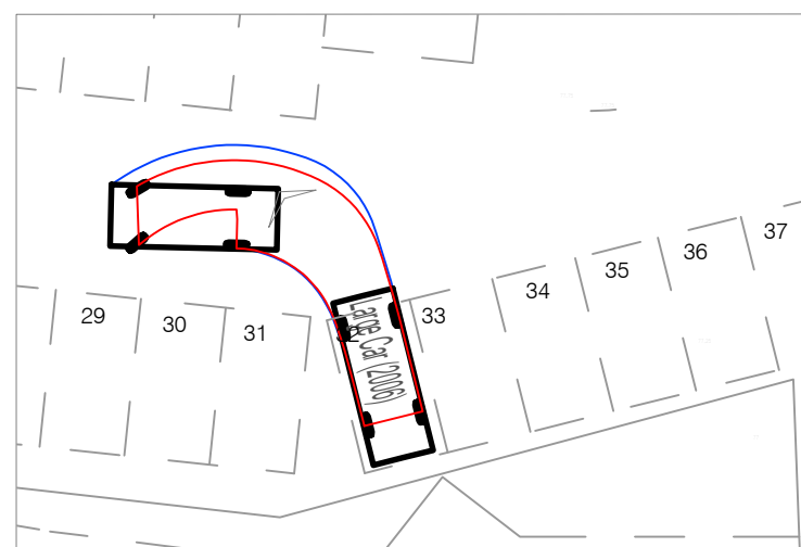
LARGE CAR EXITING SPACE 32
