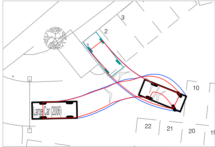
LARGE CAR ENTERING SPACE 1
