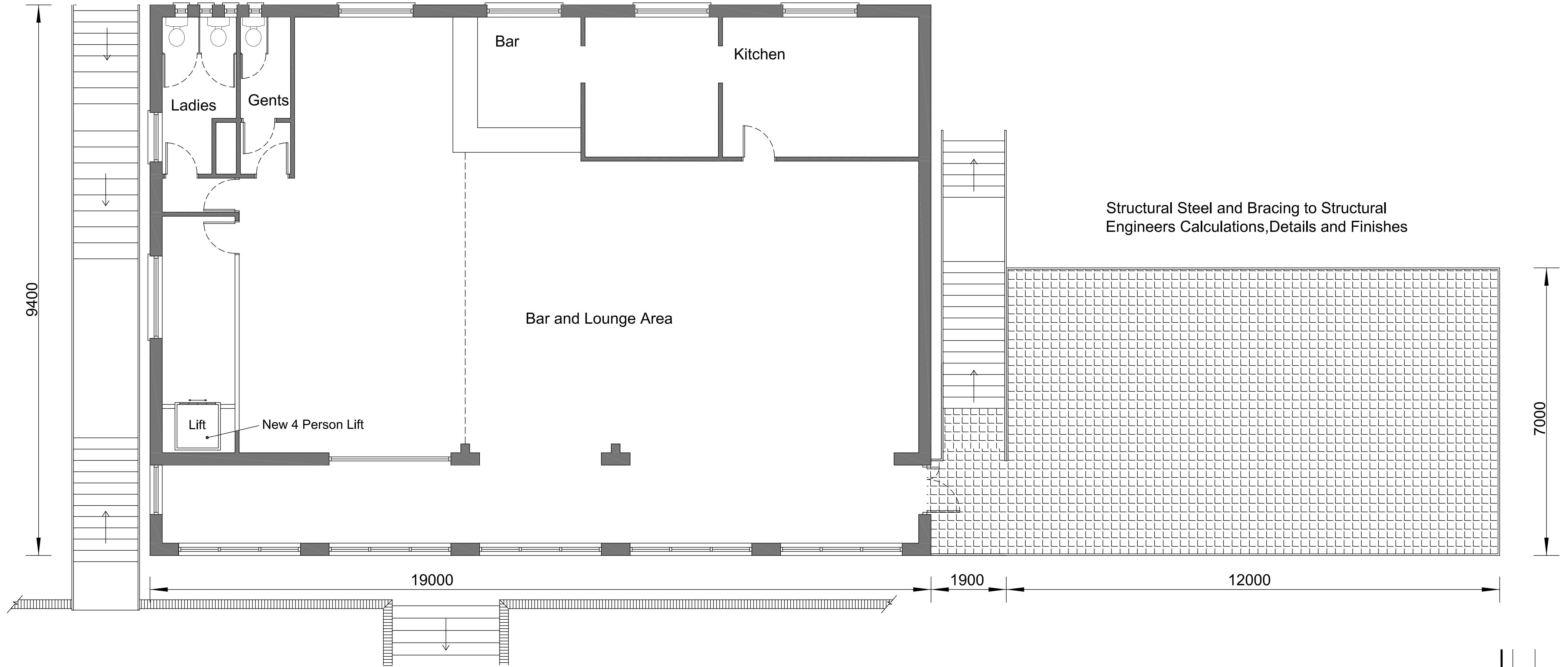
Proposed First Floor
