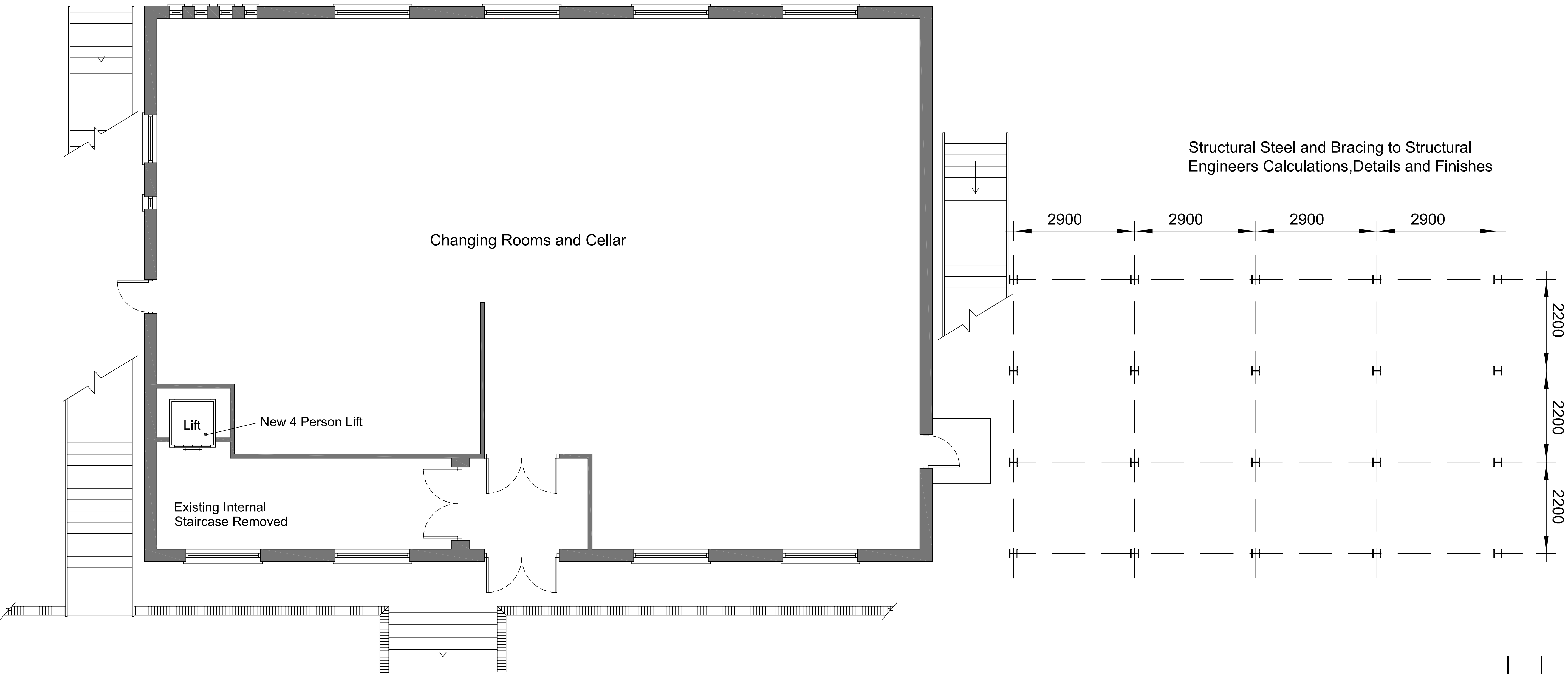
Proposed Ground Floor
