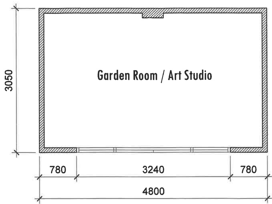
Proposed Floor Layout Plan
