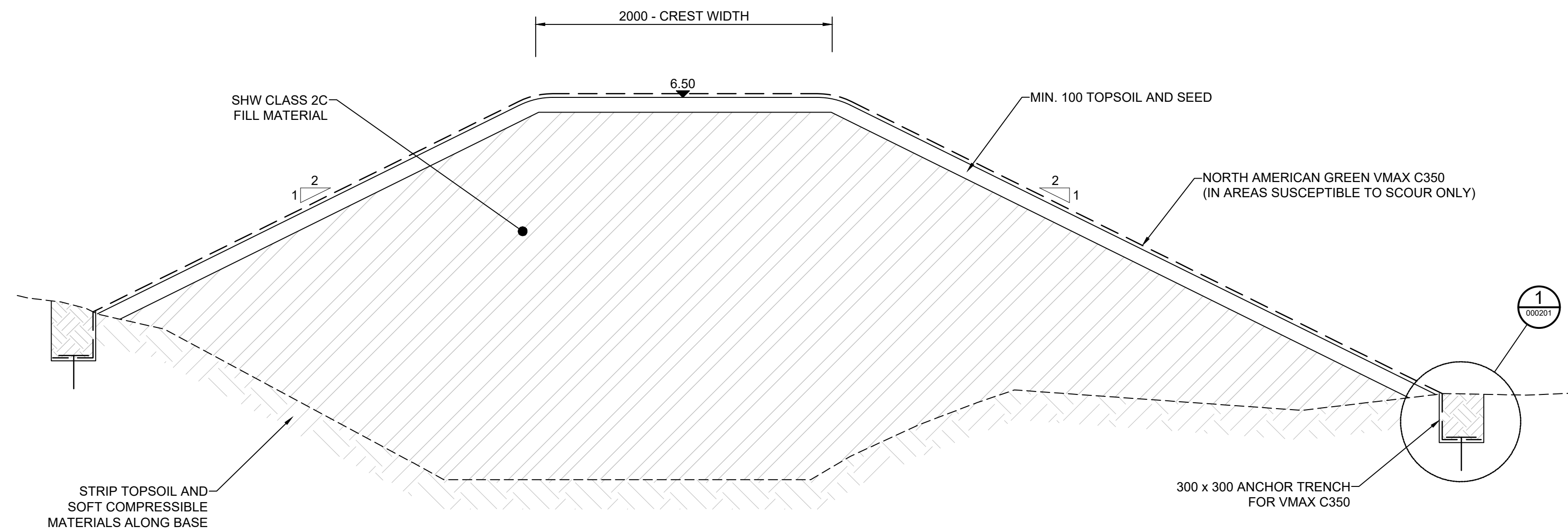
TYPICAL CROSS-SECTION THROUGH EARTH BUND
