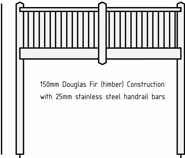
Existing Balcony front view 1/50 scale
