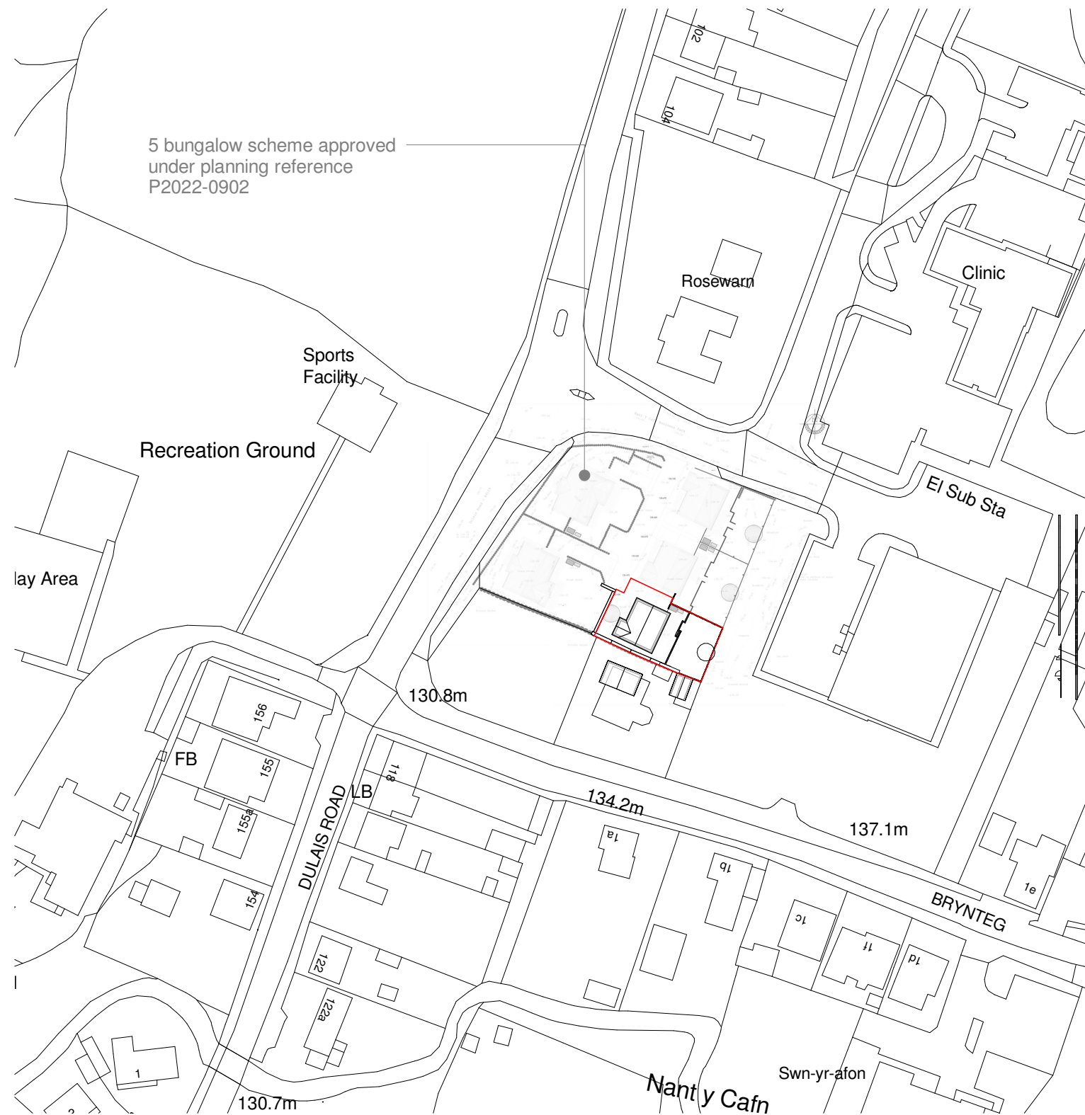
LOCATION PLAN 1 : 1250
