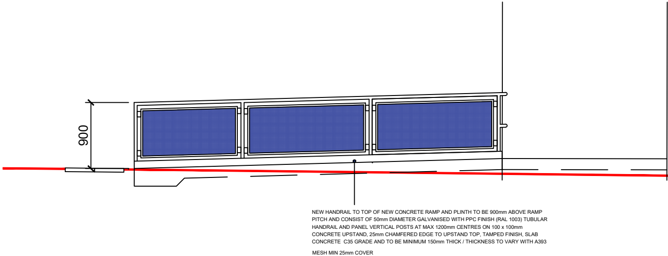
SECTION THROUGH NEW 1:15 RAMP
