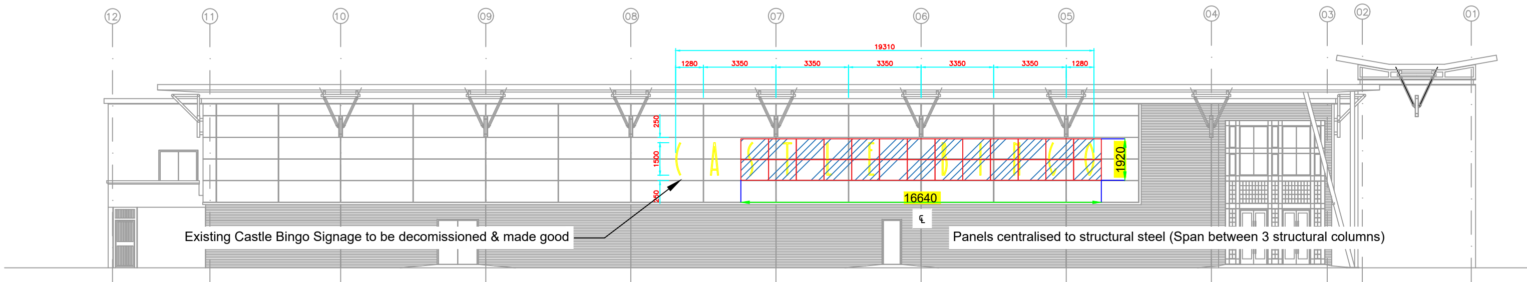
CASTLE BINGO - SOUTH WEST FACING ELEVATION (Replacement of External lettering for LED Display) 16x2 32 PANELS - 16640mm x 1920mm (Based on ABSEN [A0621-1280x960 ] Panels)
