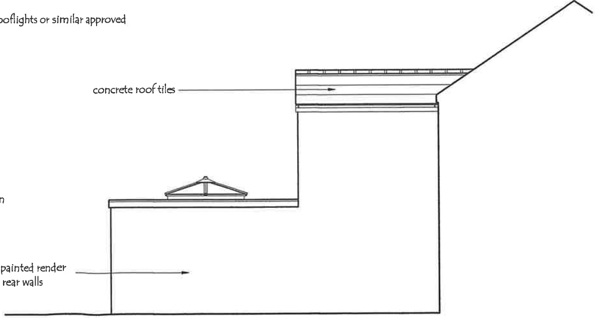
Proposed Side Elevation ( from No. 18 )
