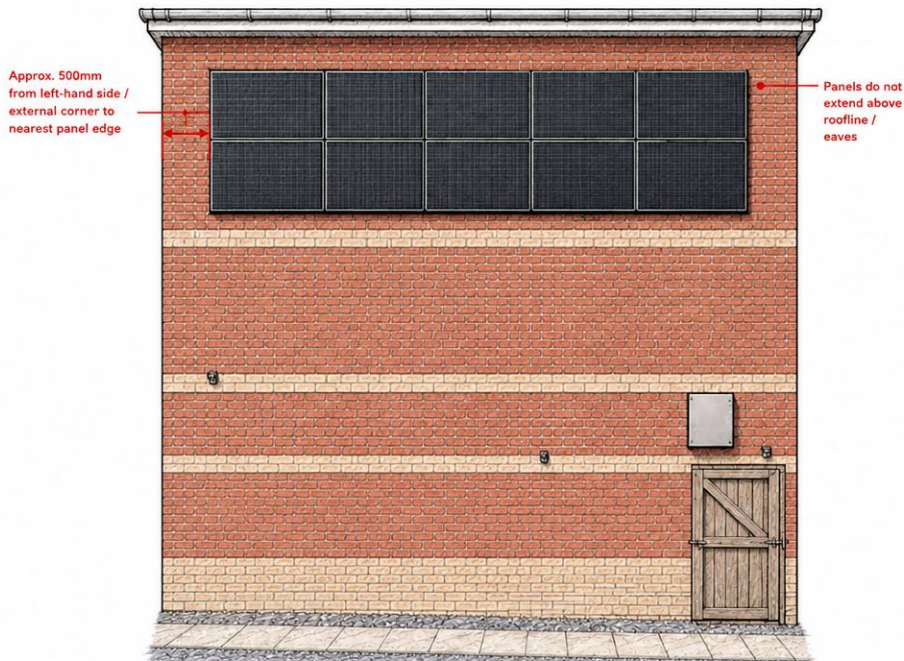
Side elevation (wall-mounted PV array) 10 no. PV panels - 2 rows of 5
