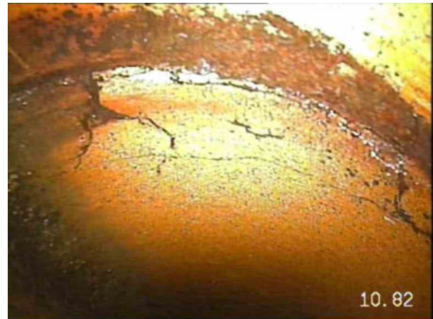
8, 00:04:26, 10.82 m Fracture, longitudinal at joint at 9 o'clock
