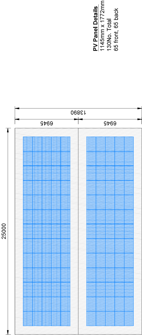
Roof Plan 1:100
