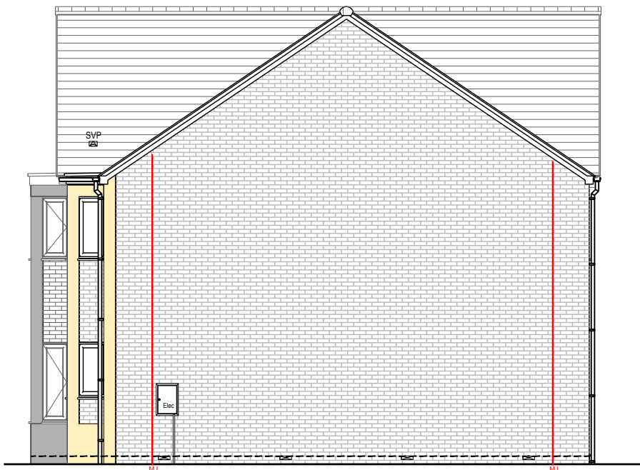
Right Elevation Plot 18 (HT A) - Handed
