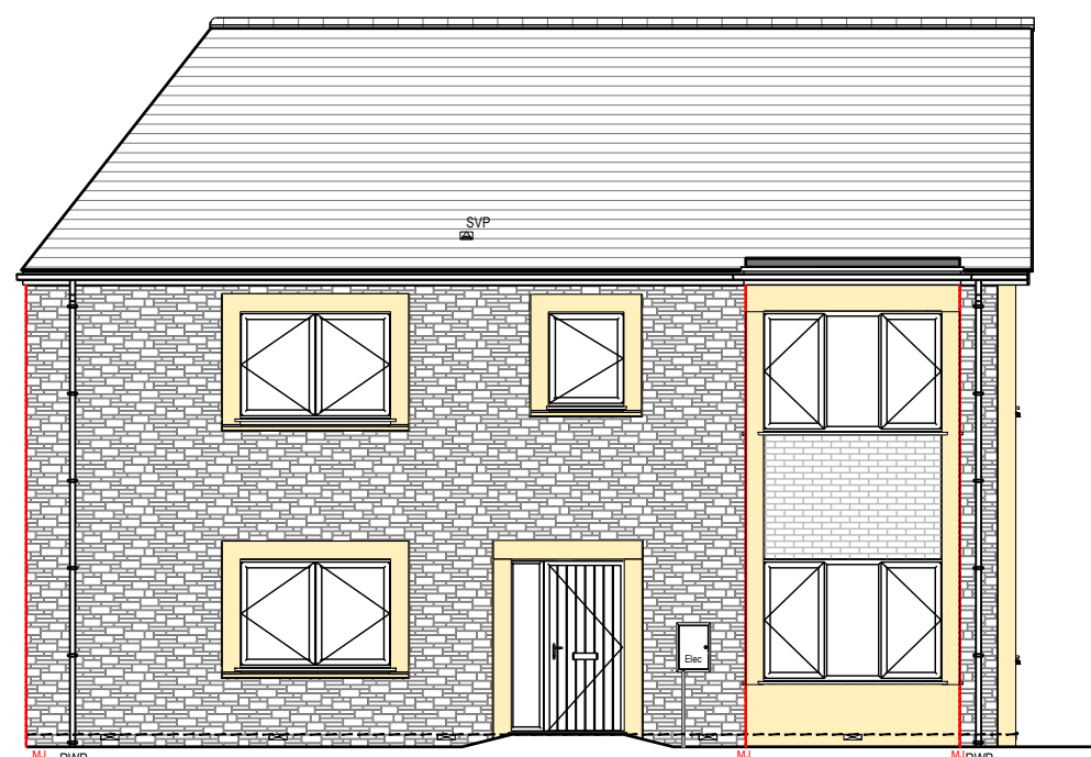
Front Elevation Plots 5 & 6 (Walk-Up Apt B) - As
