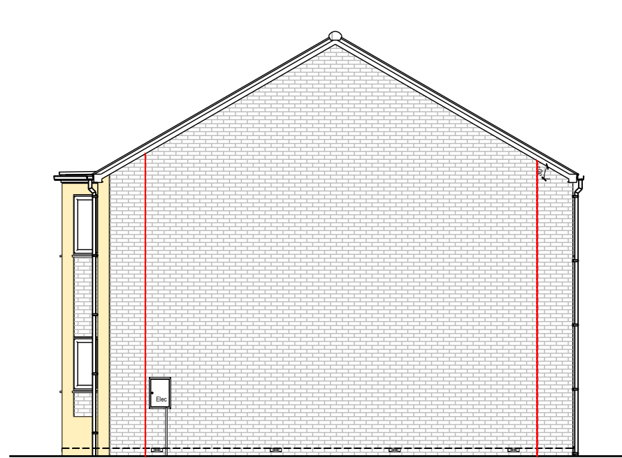
Right Elevation Plot 16 (HT A) - Handed
