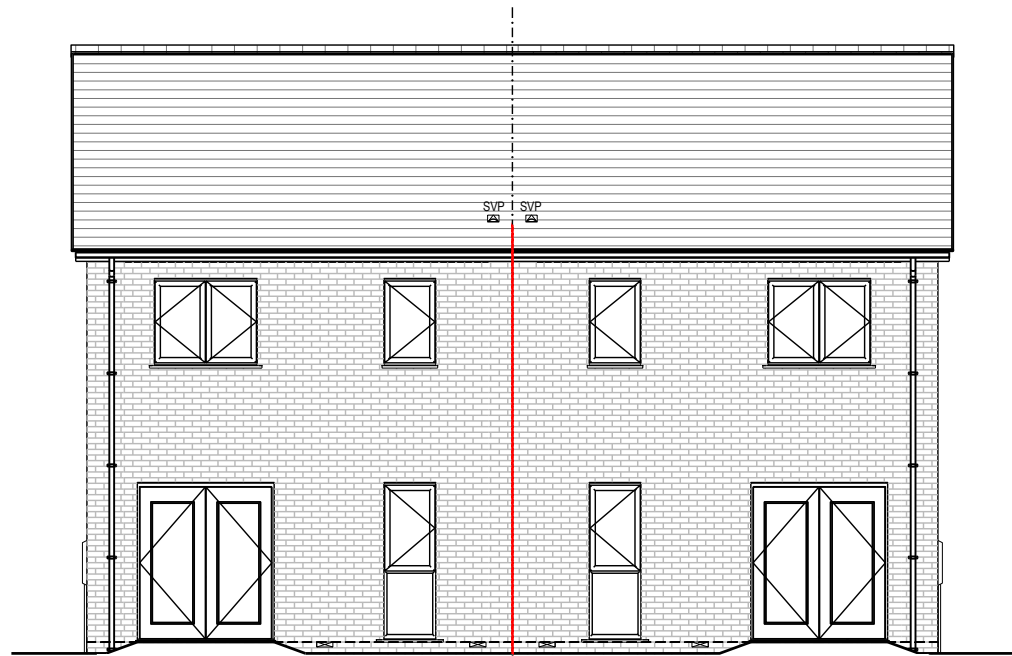
Rear Elevation Plot 16 (HT A) - Handed
