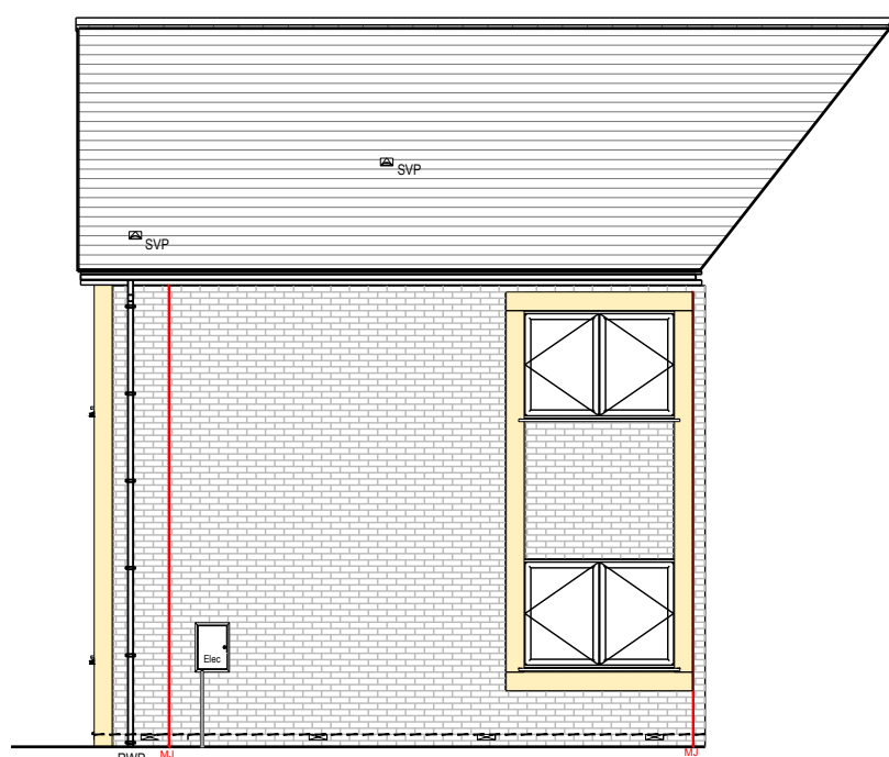
Rear Elevation Plots 5 & 6 (Walk-Up Apt B) - As
