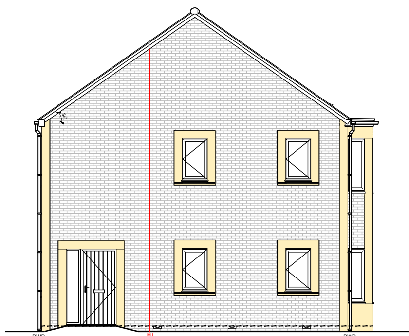
Left Elevation Plots 3 & 4 (Walk-Up Apt B) - Handed
