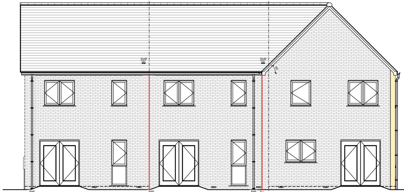
Rear Elevation Plot 18 (HT A) - Handed
