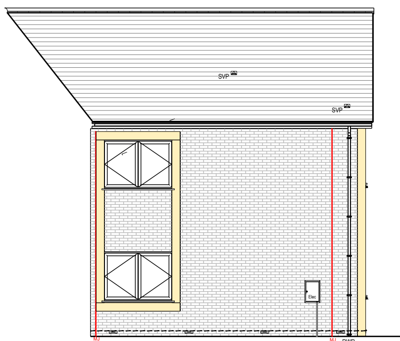
Rear Elevation Plots 3 & 4 (Walk-Up Apt B) - Handed
