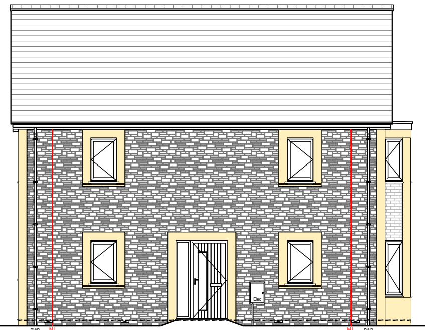
Left Elevation Plot 20 (HT C) - As
