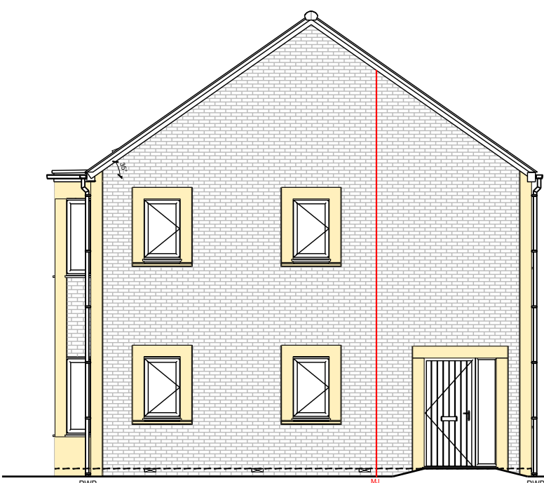
Right Elevation Plots 5 & 6 (Walk-Up Apt B) - As
