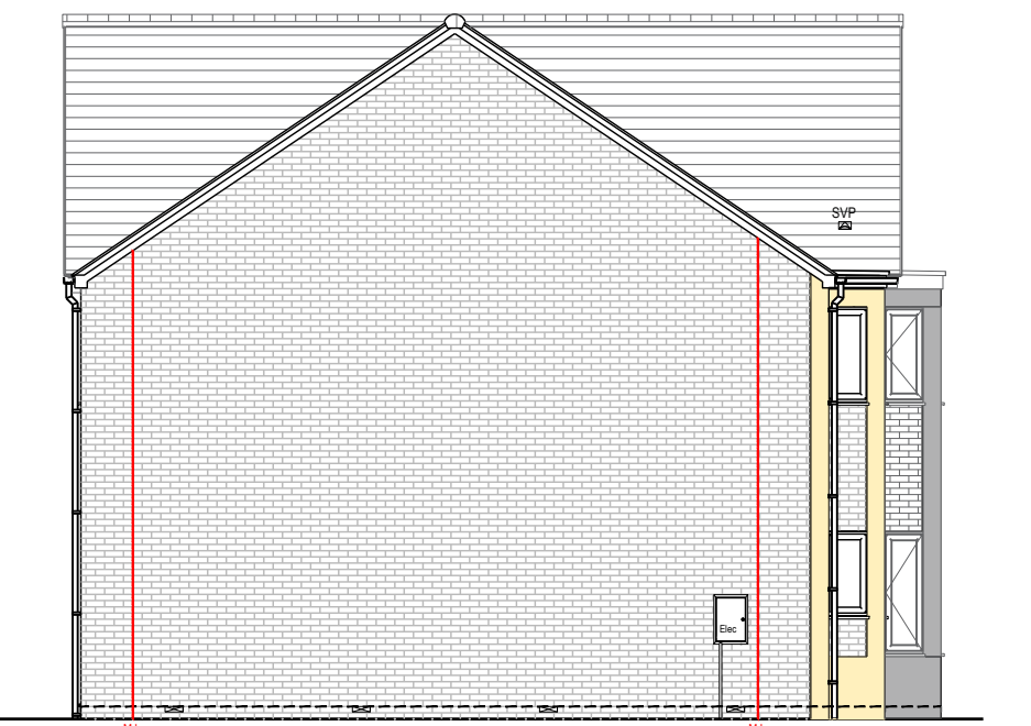
Left Elevation Plot 9 (HT A) - As
