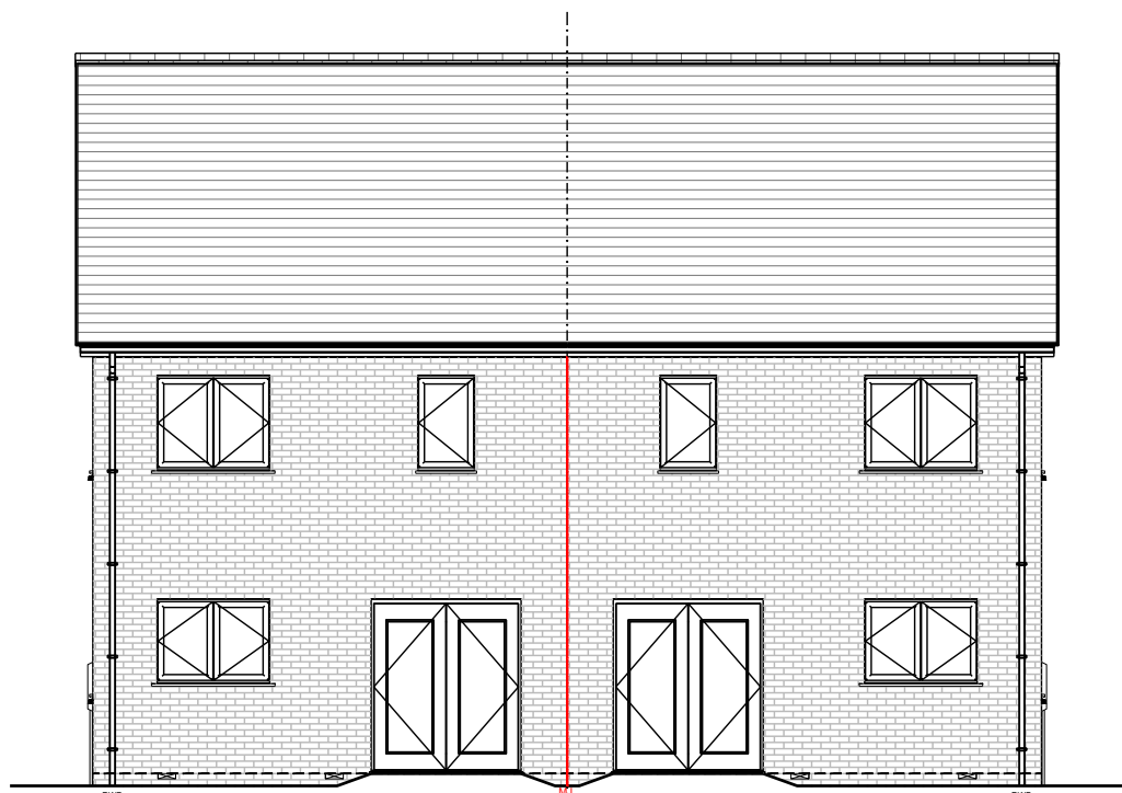
Rear Elevation Plots 2 & 41 (HT B) - Handed Plots 1 & 42 (HT B) - As
