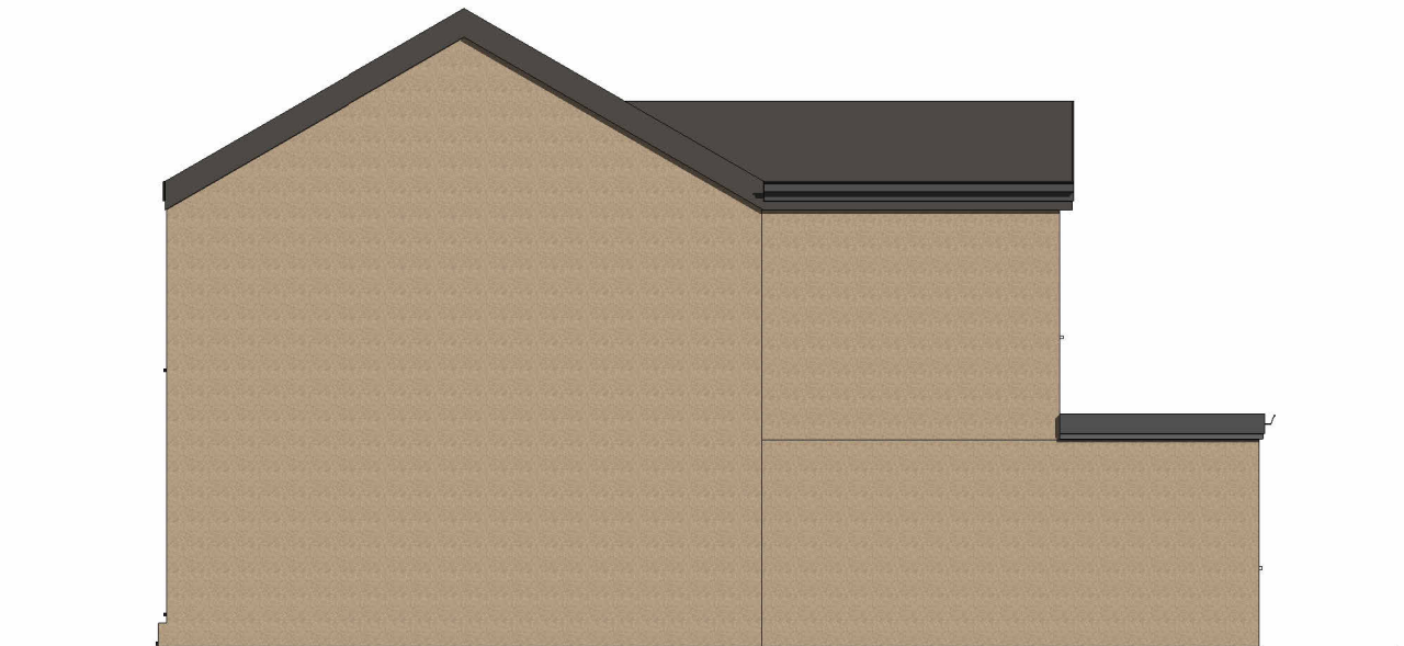
4 Proposed Side Elevation (2) 1 : 100
