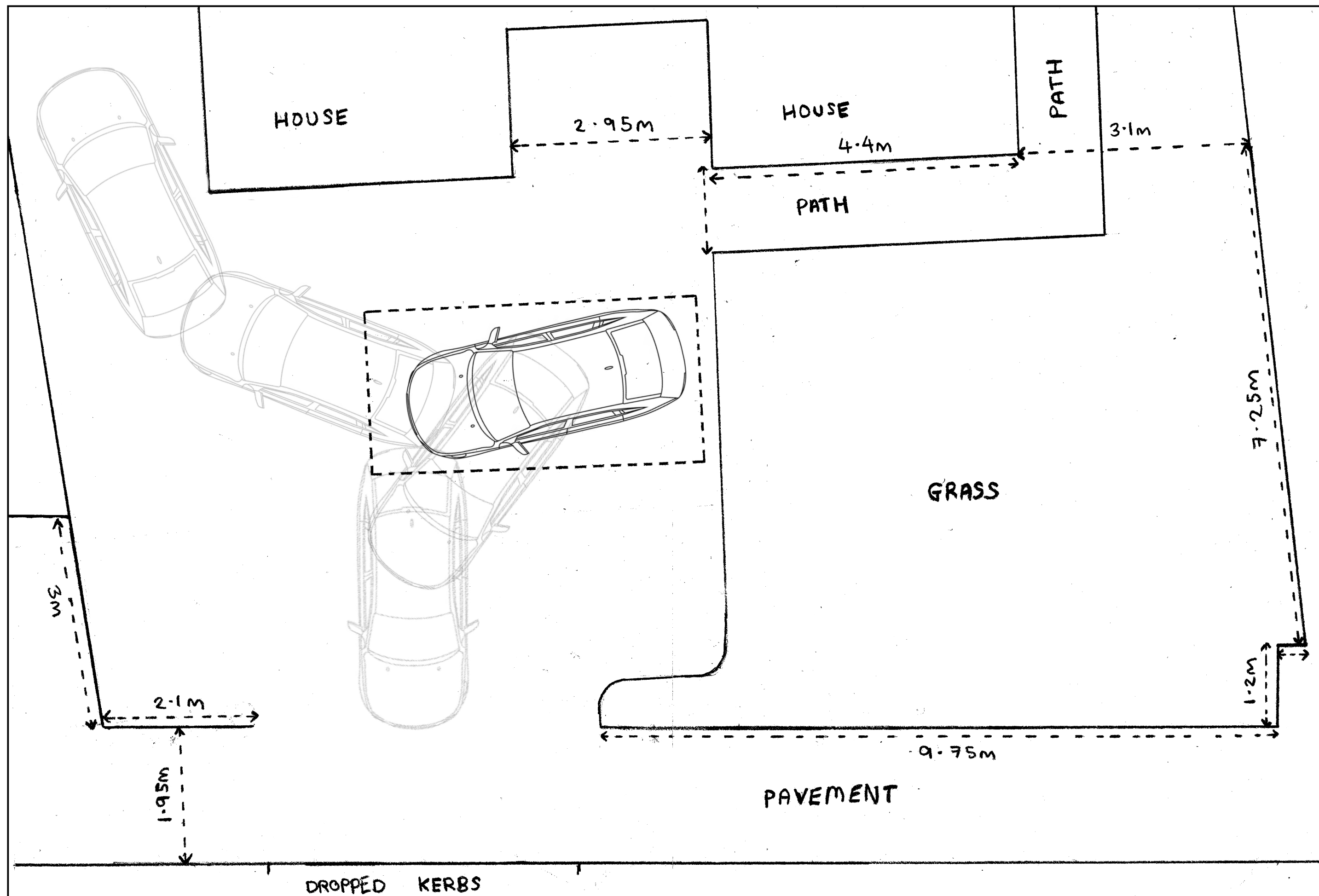
Site plan (Parking and access) 6 Commercial Road, Rhydyfro, Swansea SA84SL
