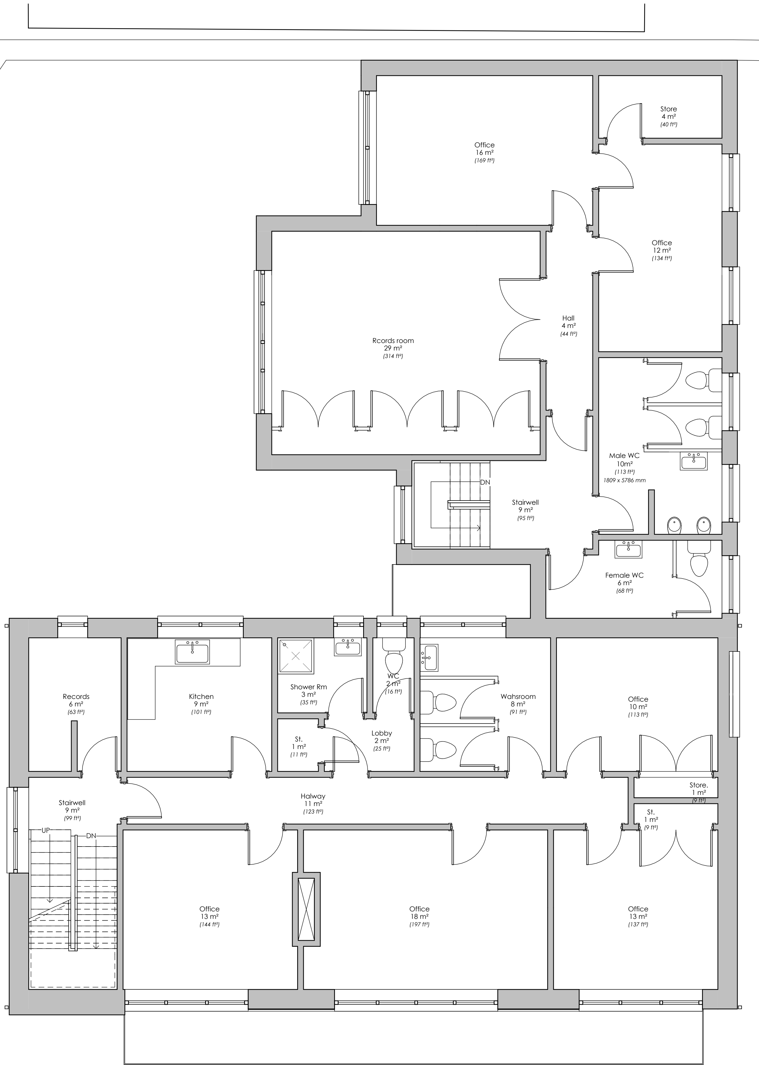
View No. 01 Existing First Floor 1:50
