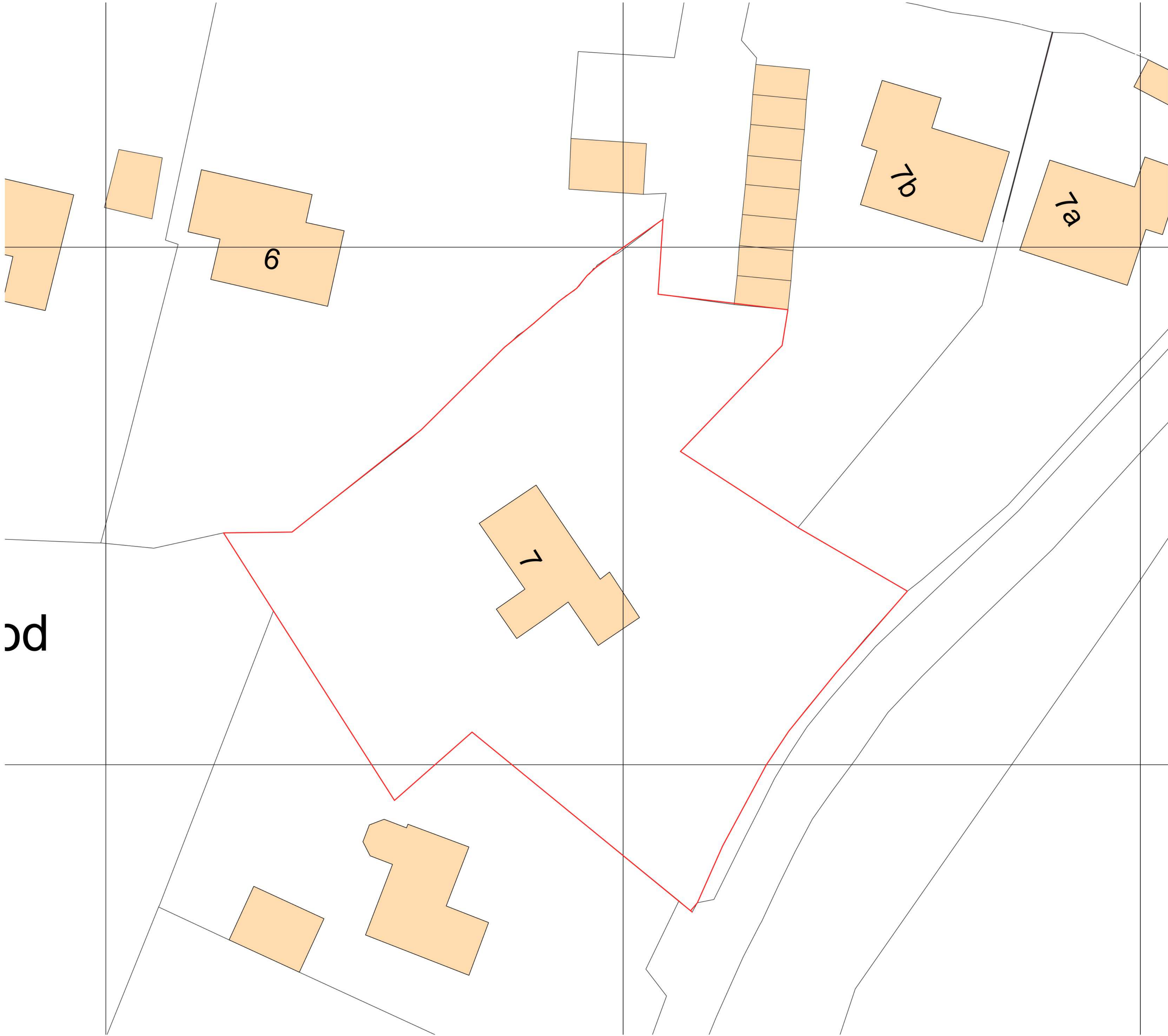
Site Block Plan 1:200
