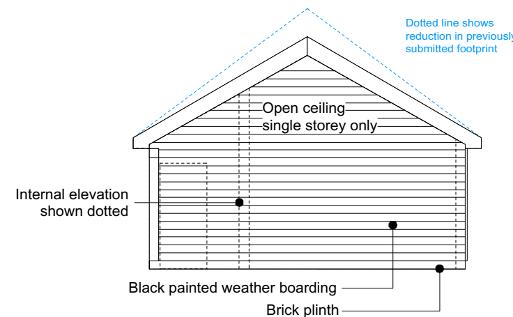
Proposed East Elevation 1:100
