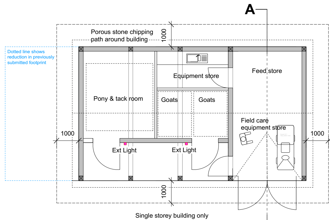
Proposed Plan 1:100
