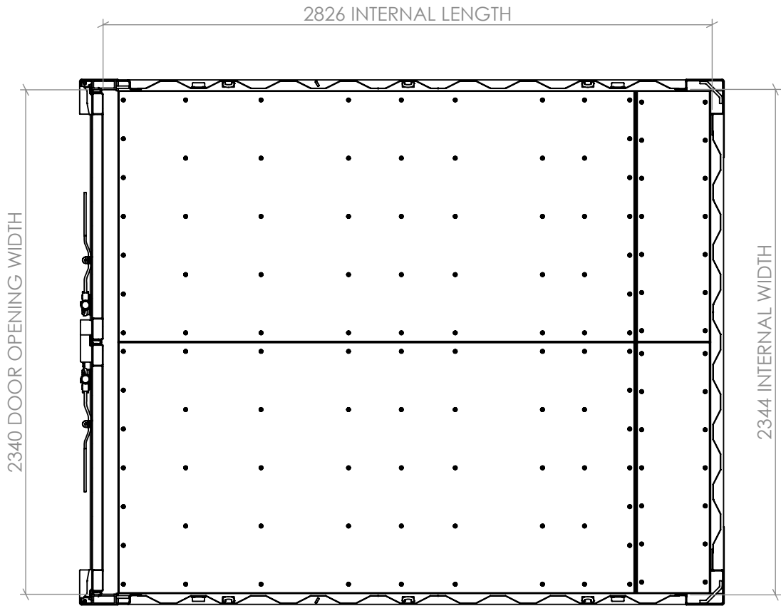
SECTION A-A FLOOR PLAN
