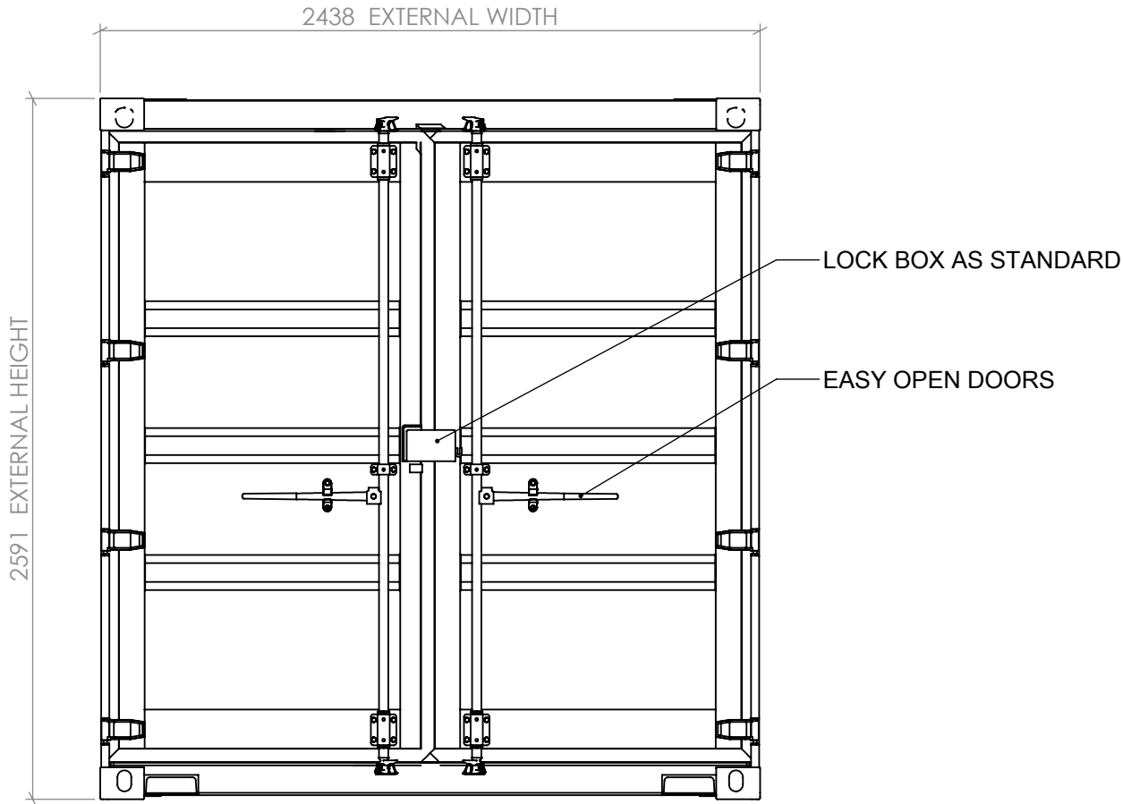
REAR (DOOR) END
