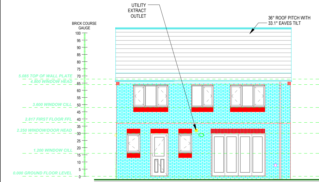
REAR ELEVATION
