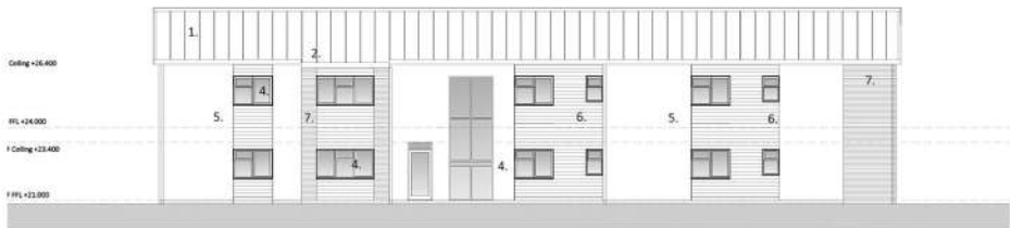
Proposed Rear Elevation - South East Previously consented scheme
