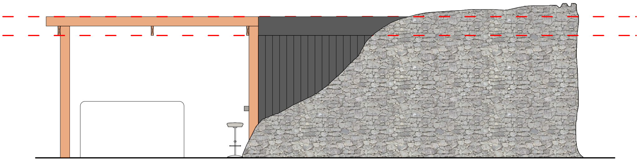
Rear Elevation 1:50
