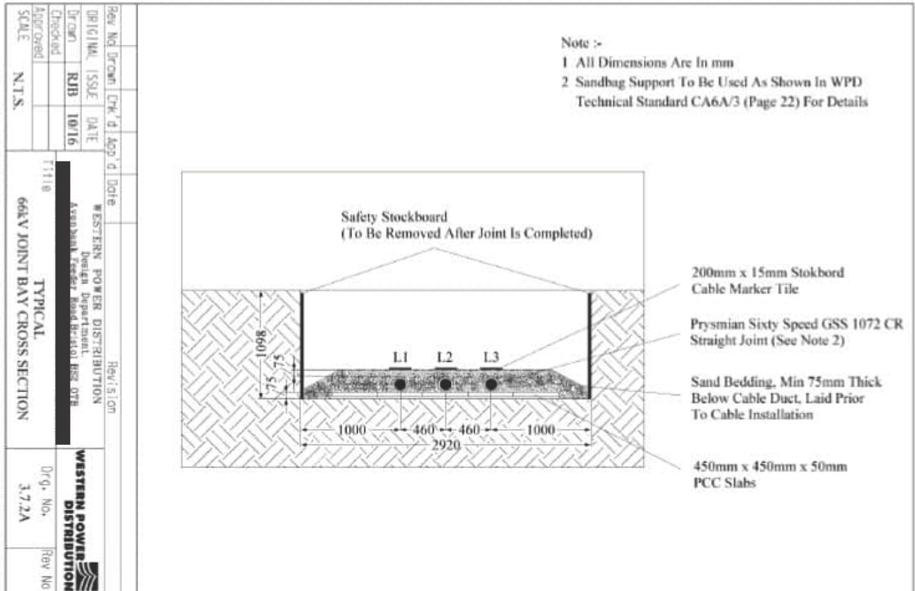
Figure 6 66kV Joint Bay Layout (Sheet 2 of 2)
