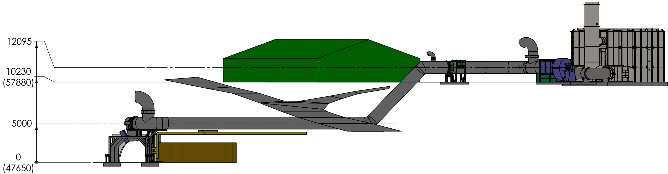
SIDE ELEVATION
