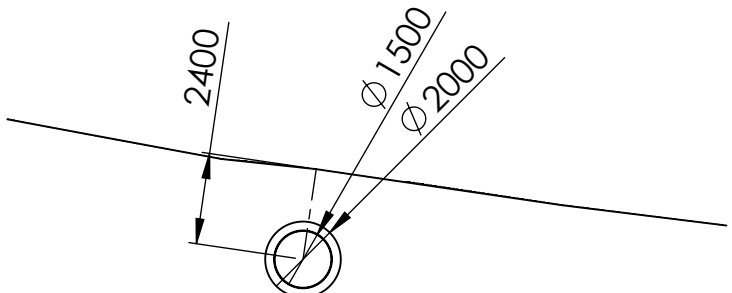
ENLARGED SECTION A-A perpendicular to duct
