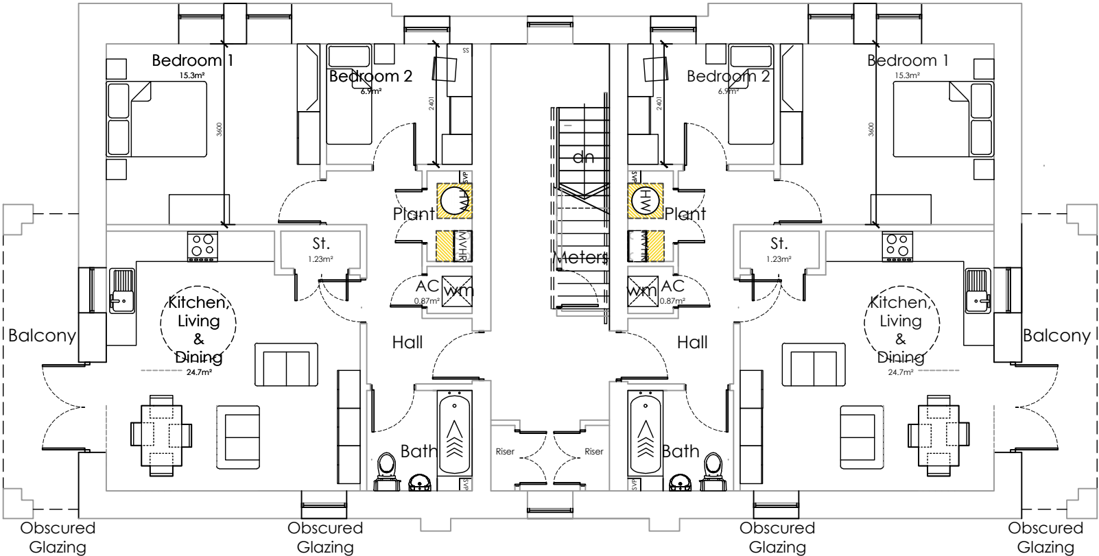
BUILDING TYPE A: FIRST FLOOR PLAN
