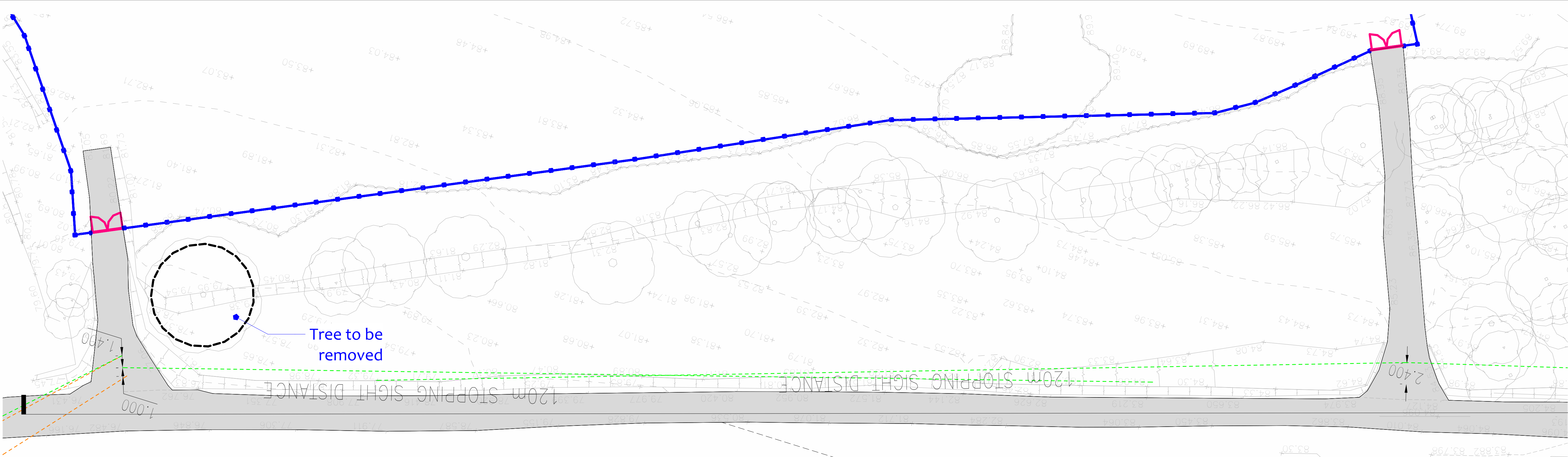
01 Boundary Plan - Access Points 1 : 250
