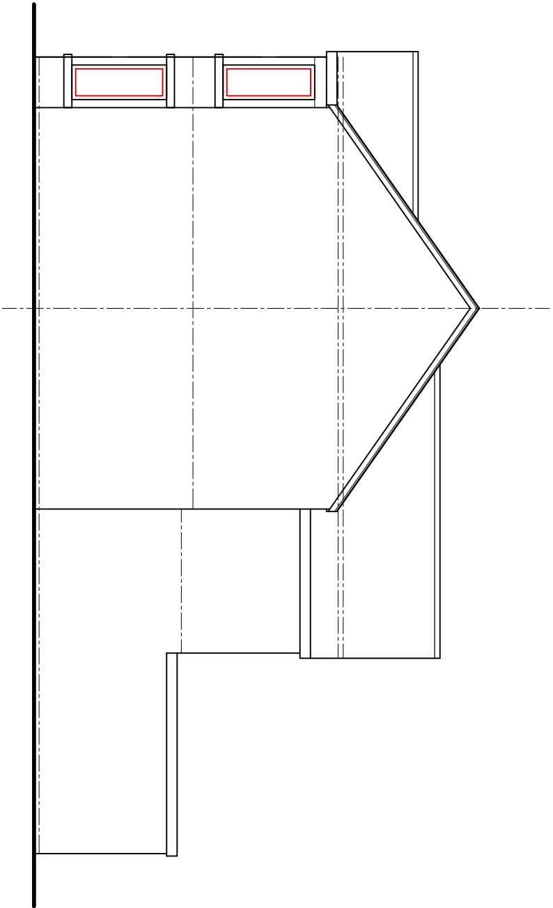
EXISTING SIDE SOUTH ELEVATION. (1:100)
