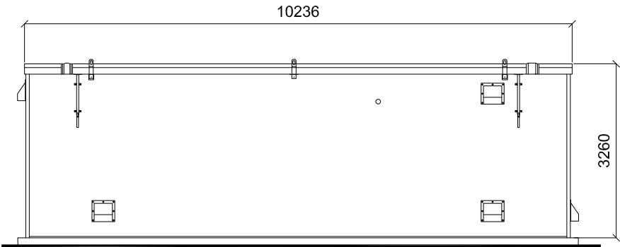
REAR ELEVATION
