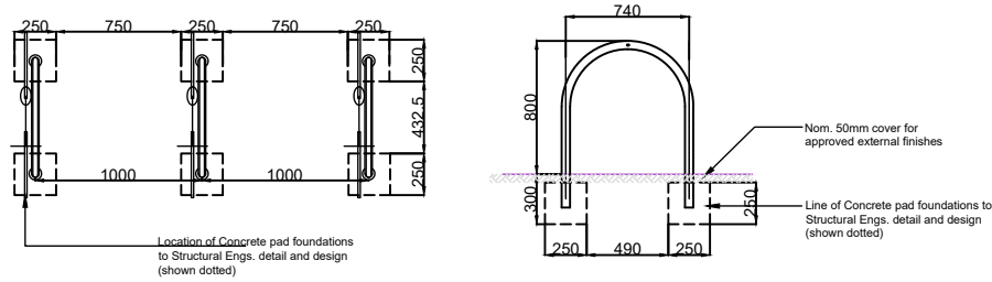
No. 6 Cycle Store Foundation Layout
