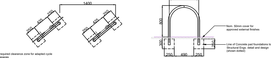
No. 4 Adapted Cycle Store Foundation Layout
