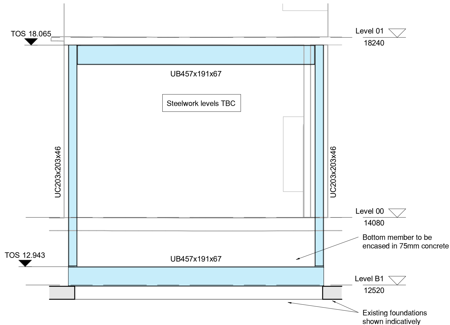
Typical 'Picture Frame' Steelwork Layout
