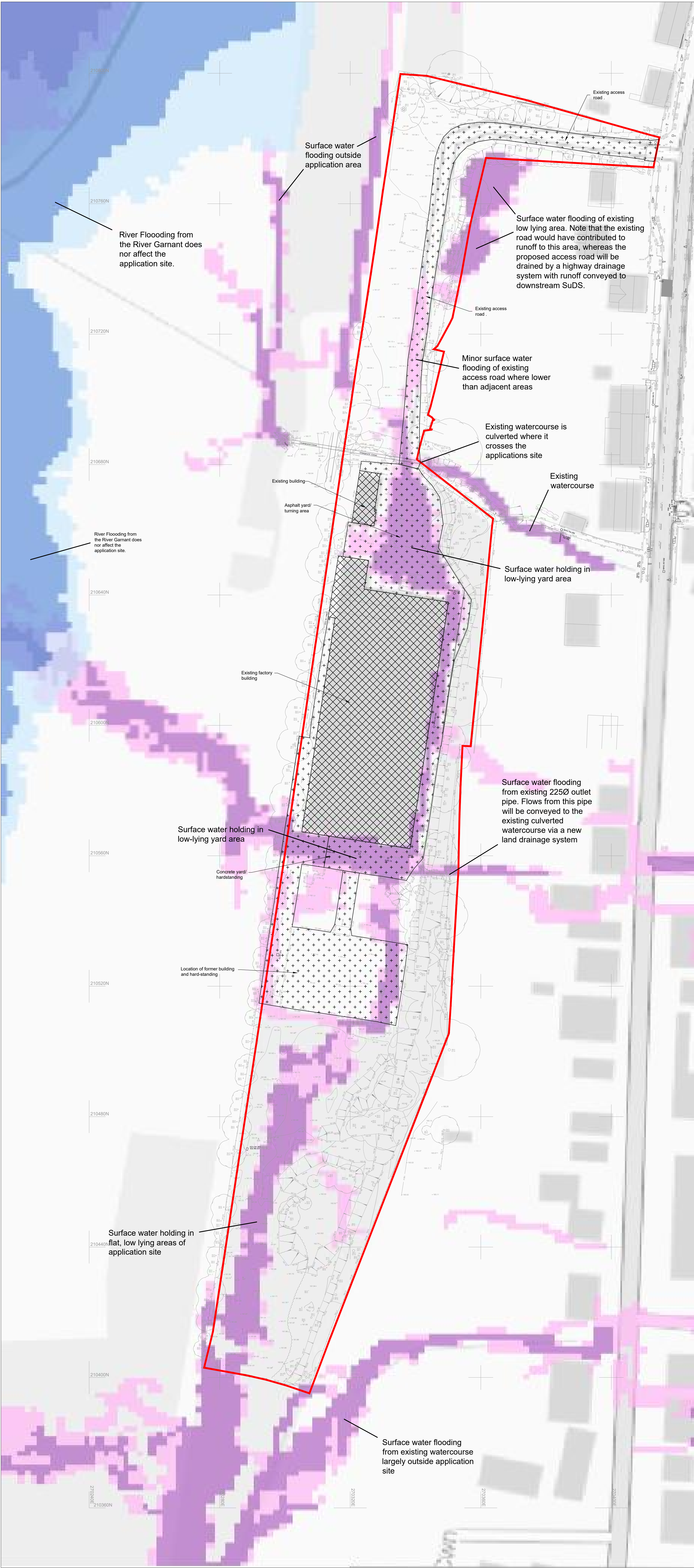
Overlay of 'NRW Flood Map for Planning' over Site Topographical Survey Scale 1:500
