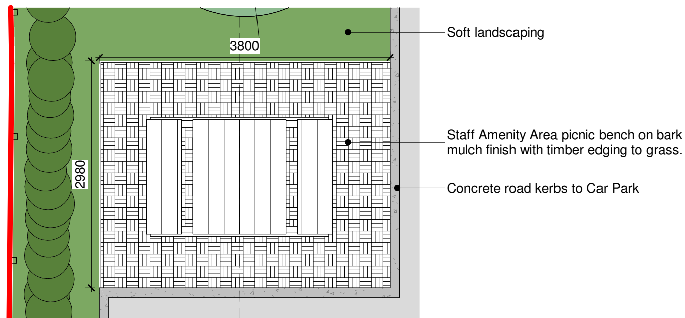
Site Layout as proposed - Staff Amenity 1 : 50
