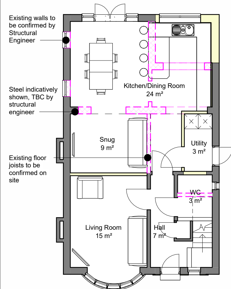
1.1 - Proposed Ground Floor 1 : 100
