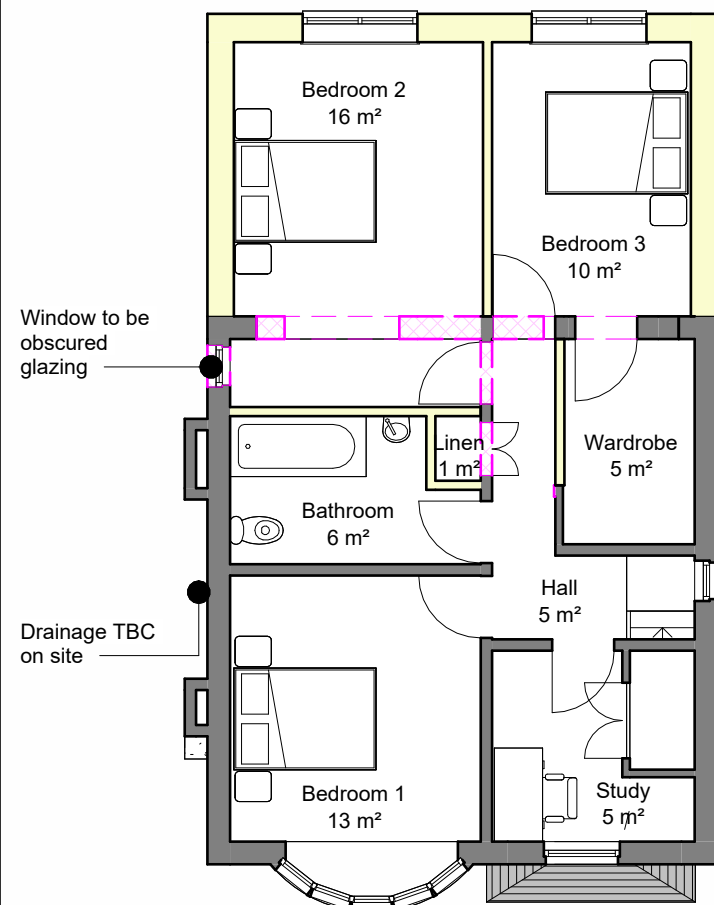
2.1 - Proposed First Floor 1 : 100
