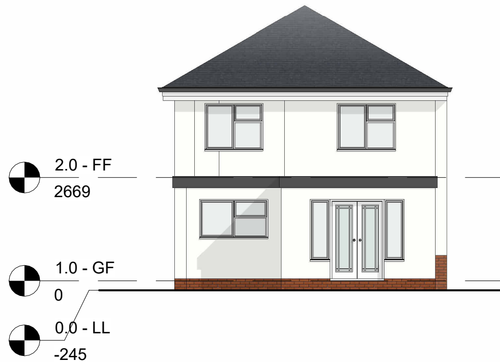
4 Existing Rear Elevation 1 : 100
