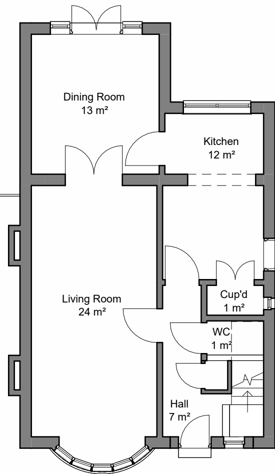
1 1.0 - Existing Ground Floor 1 : 100
