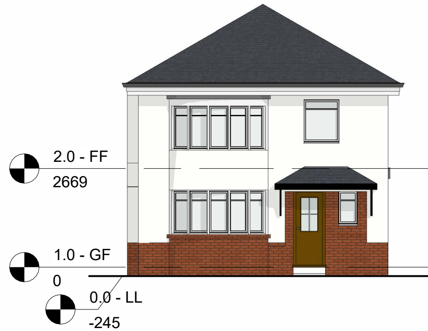
3 Existing Front Elevation 1 : 100
