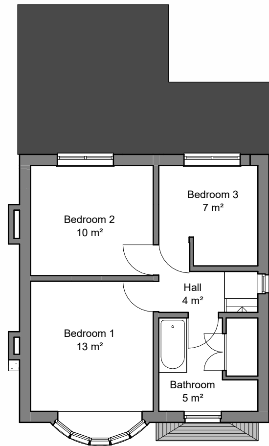
2 2.0 - Existing First Floor 1 : 100
