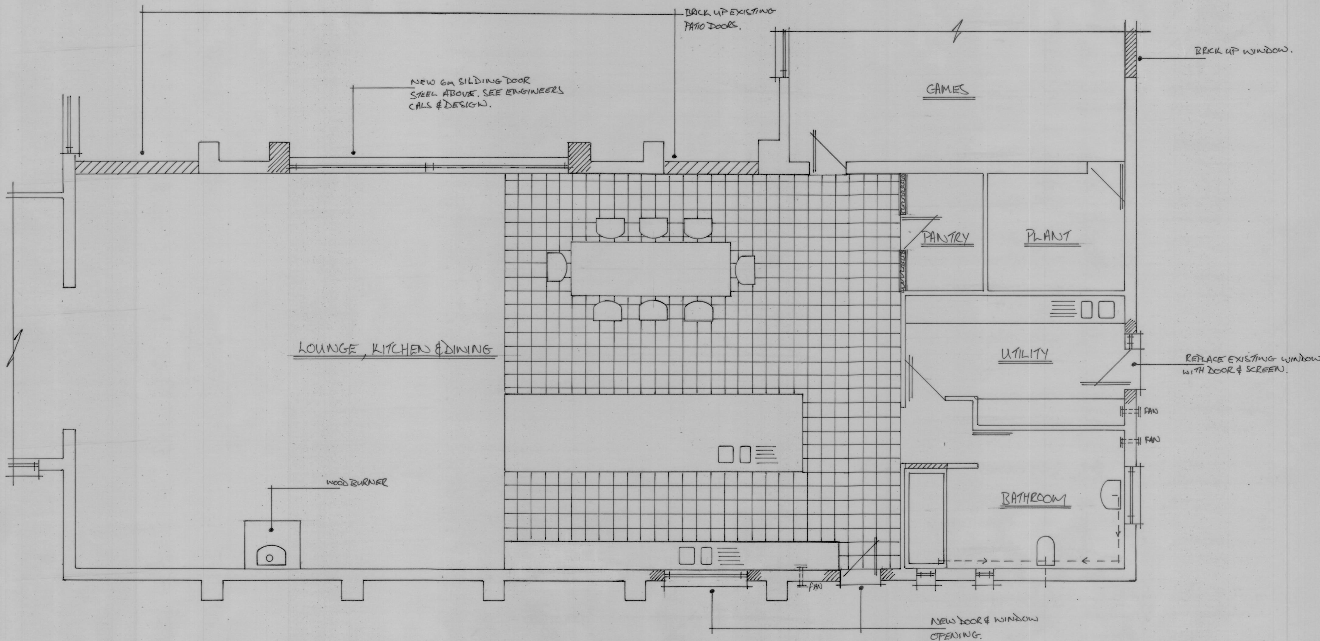
PROPOSED GROUND FLOOR (1:50)
