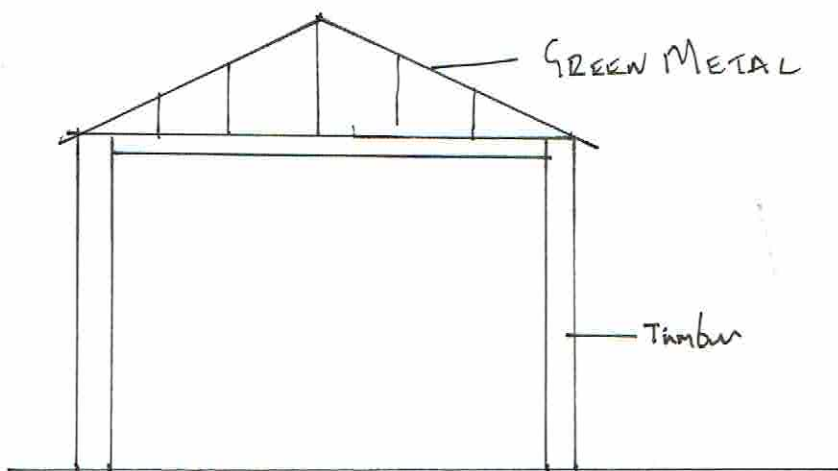
SIDE ELEVATIONS GAZIBO
