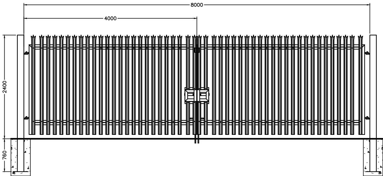
ELEVATION / SECTION
