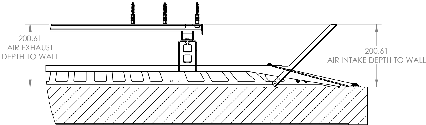
DETAIL B
