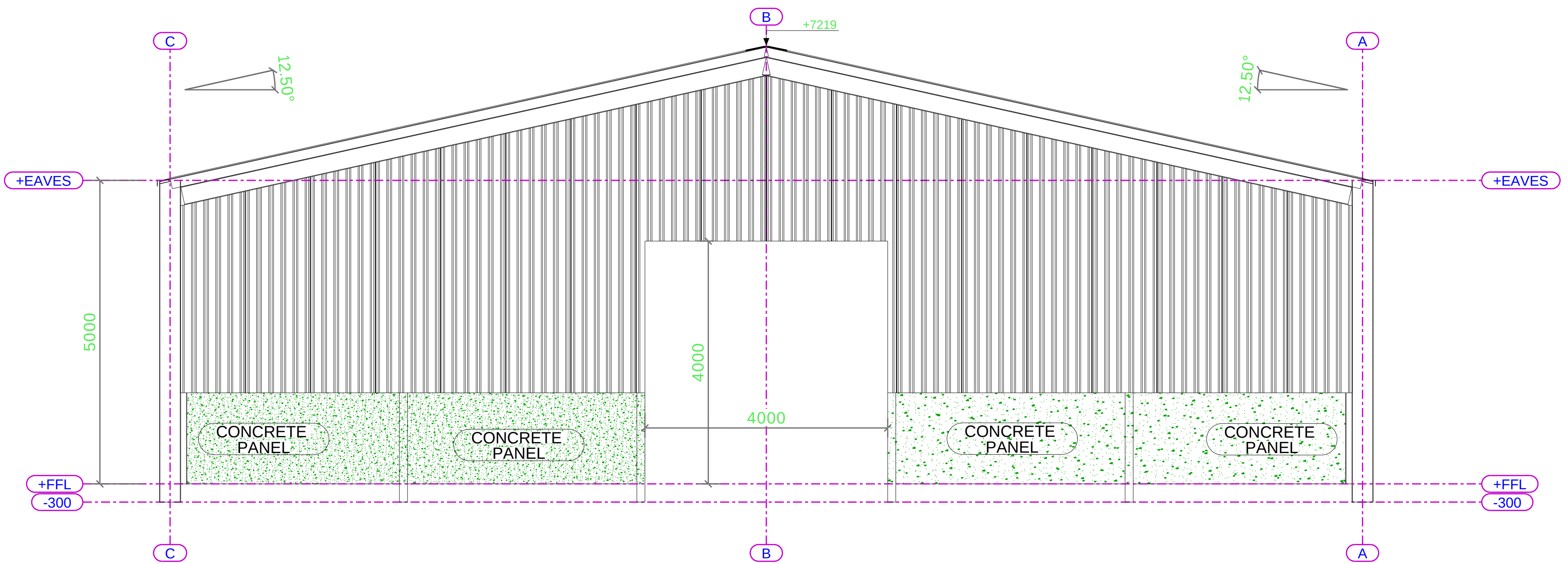
Elevation on Line 8 Scale 1 : 50 @ A0
