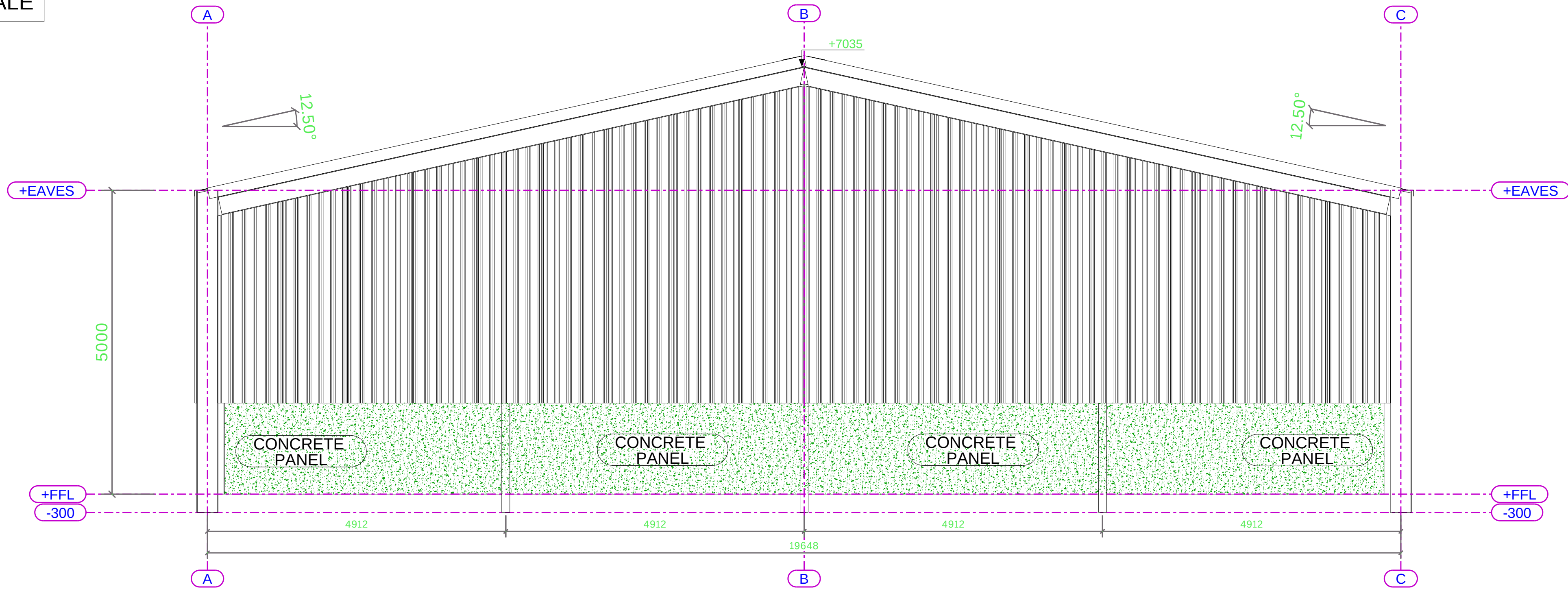
Elevation on Line 1 Scale 1 : 50 @ A0
