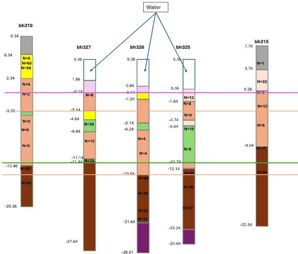
Figure 3-8 Ground conditions in Area A5
