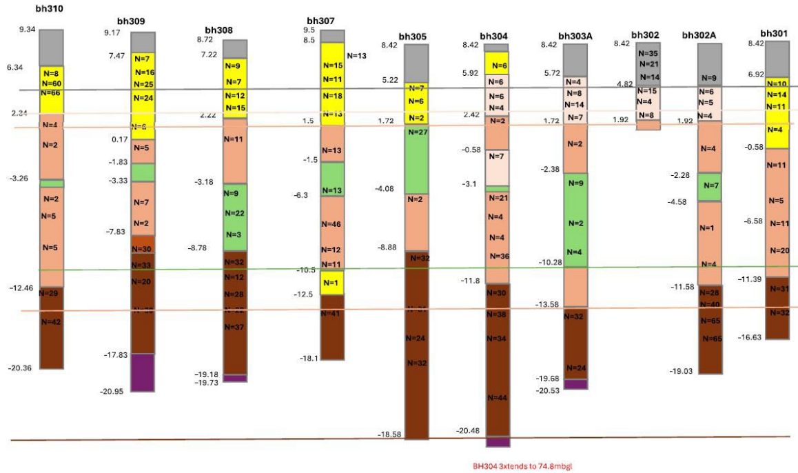
Figure 3-5 Ground conditions in Area A2
