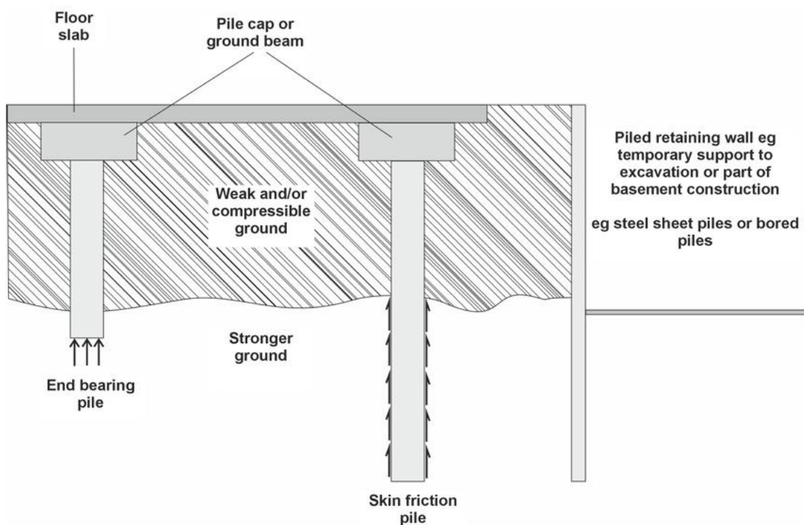
Figure 4-1 Examples of pile foundations (reproduced from Claire, 2025)
