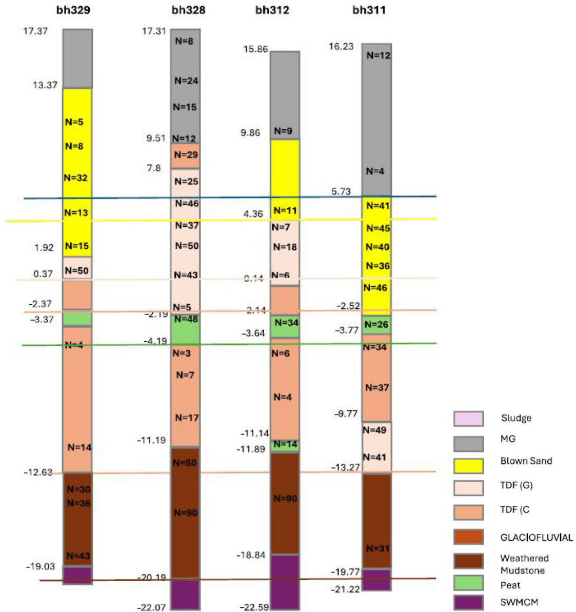
Figure 3-4 Ground conditions in Area A2. Note TDF- G is granular and TDF-C is cohesive
