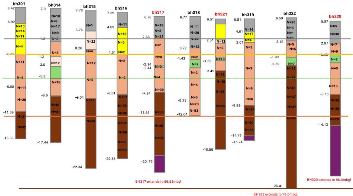
Figure 3-6 Ground conditions in Area A3
