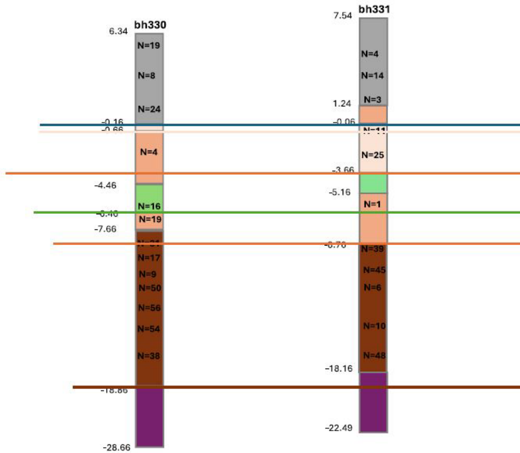
Figure 3-7 Ground conditions in Area A4
