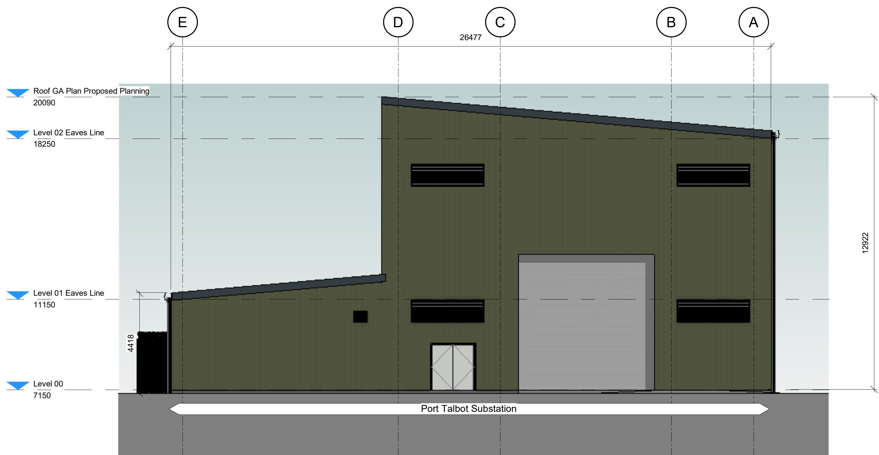
2 ZZ EastElevation Scale: 1:100
