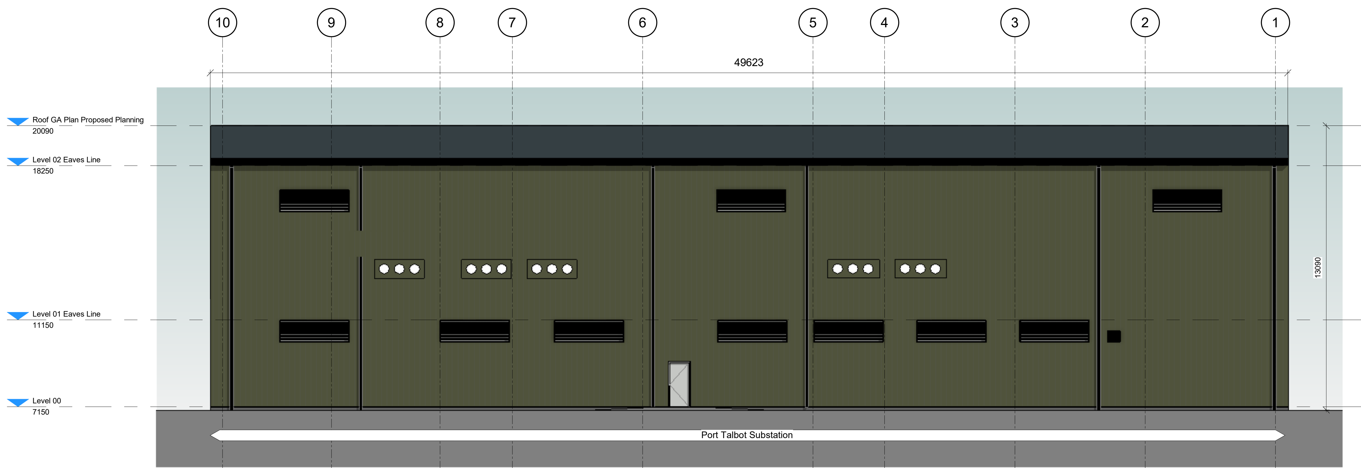
1 ZZ NorthElevation Scale: 1:100
