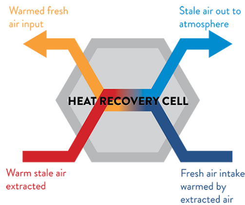
Figure 9: Diagram illustrating principle of heat recovery, property of Xpelair
