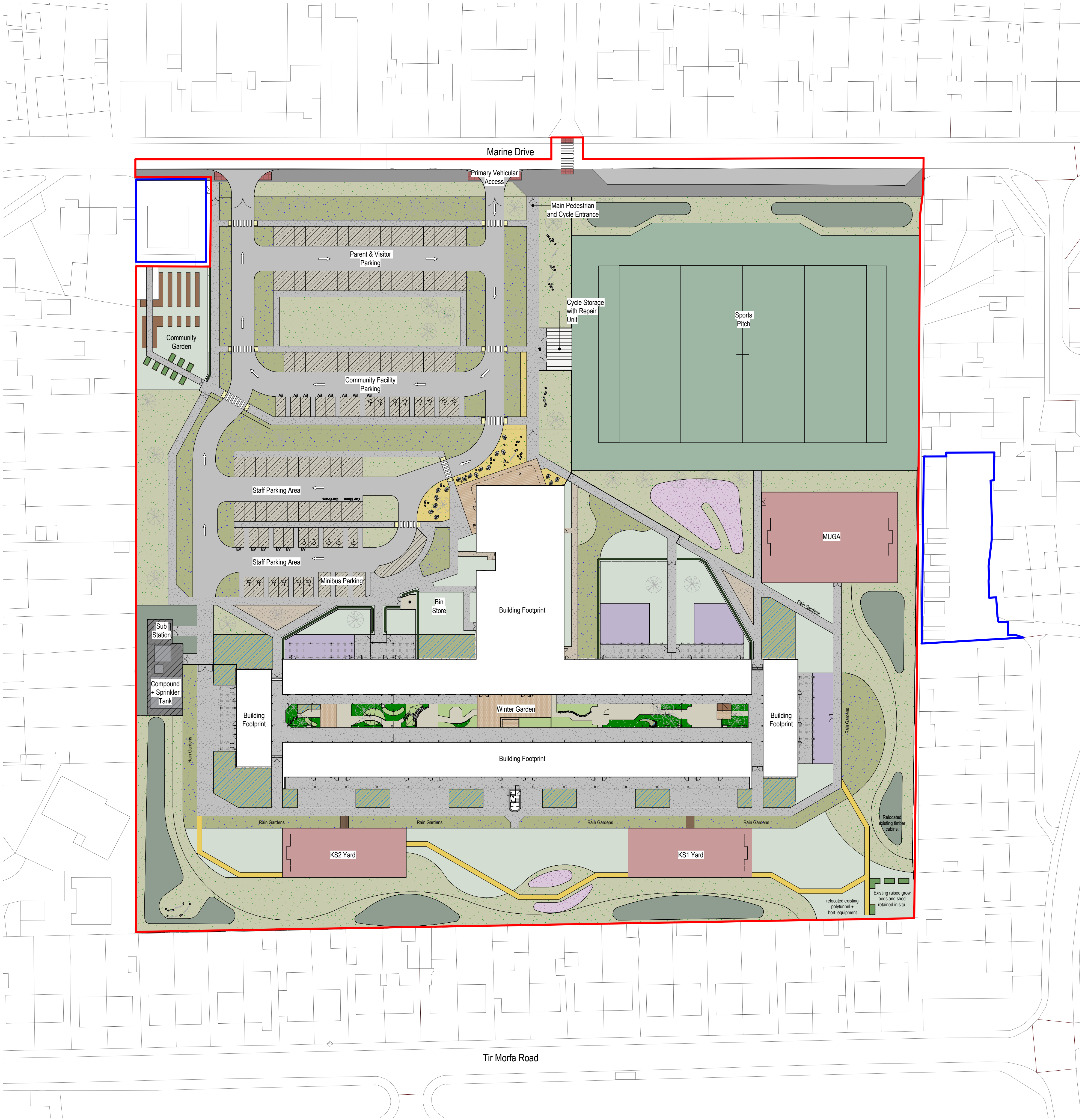
Proposed Site Block Plan 1 : 500
