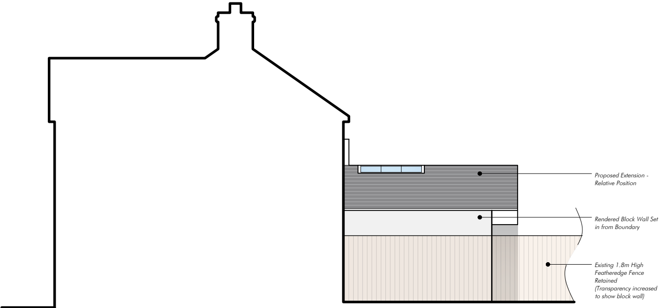
Proposed Elevation 'A' 1:100
