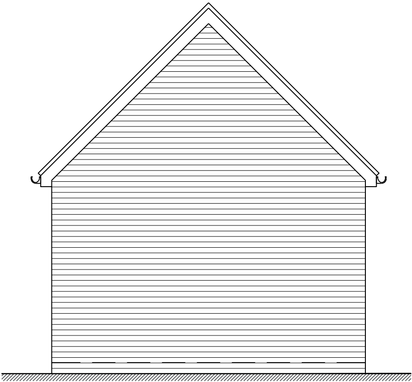
Side Elevation
